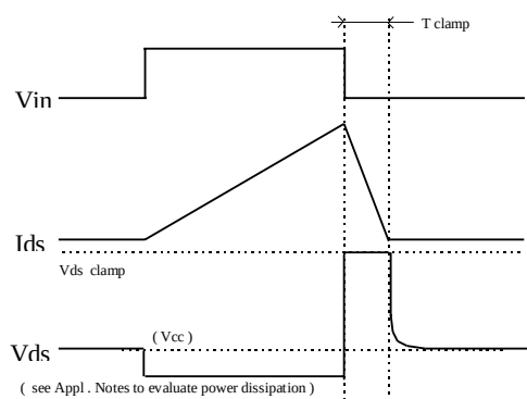
Figure 3 - Active clamp waveforms
