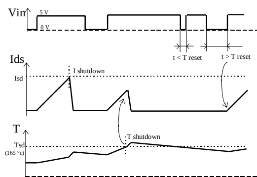
Figure 1 - Timing diagram
