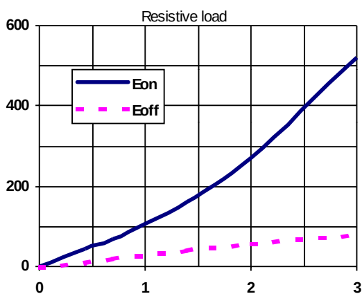
Figure 14 - E_{on} , E_{off} (μJ) (A) Vs I_{out} (A)
