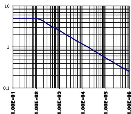
Figure 10 - Max. Iout (A) Vs Load Inductance (μH)
