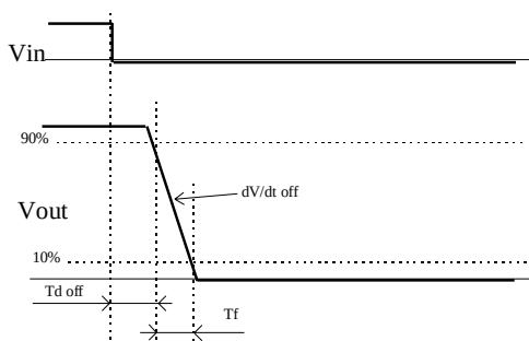
Figure 4 - Switching times definition (turn-off)
