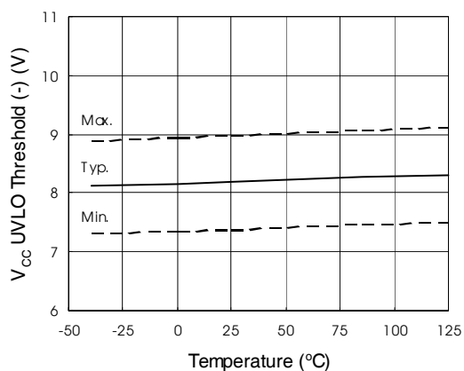
Figure 24. V_{CC} Undervoltage Threshold (-) vs. Temperature
