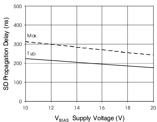
Figure 8B. SD Propagation Delay vs. Supply Voltage
