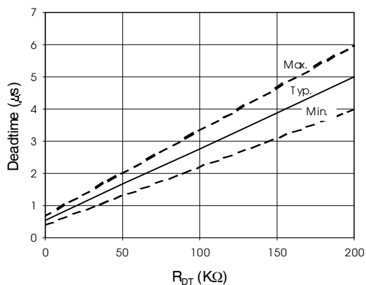
Figure 11C. Deadtime vs. RDT (IR21094 only)
