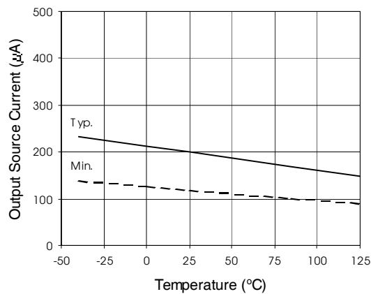
Figure 27A. Output Source Current vs. Temperature
