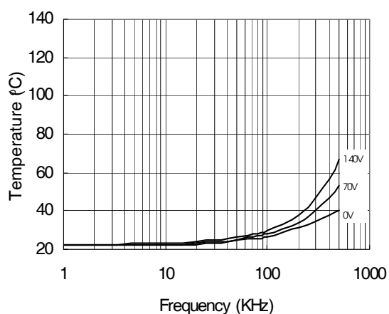
Figure 35. IR21094 vs. Frequency (IRFBC30), R_{gate}=22\Omega , V_{CC}=15V
