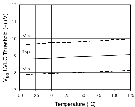
Figure 25. V_{BS} Undervoltage Threshold (+) vs. Temperature
