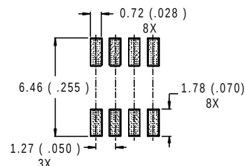
RECOMMENDED FOOTPRINT
