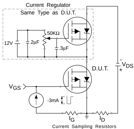
Fig 12b. Gate Charge Test Circuit
