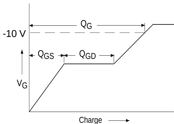
Fig 12a. Basic Gate Charge Waveform
