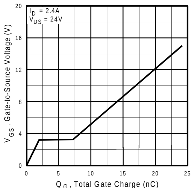
Fig 9. Typical Gate Charge Vs. Gate-to-Source Voltage
