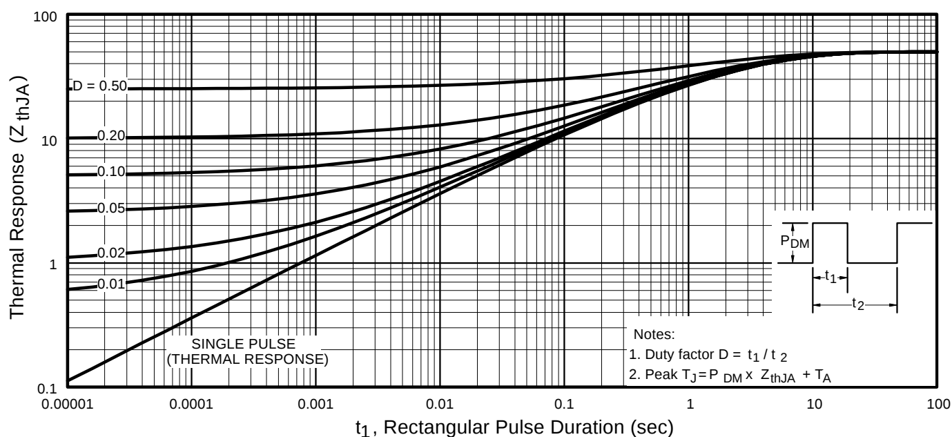
Fig 20. Maximum Effective Transient Thermal Impedance, Junction-to-Ambient
