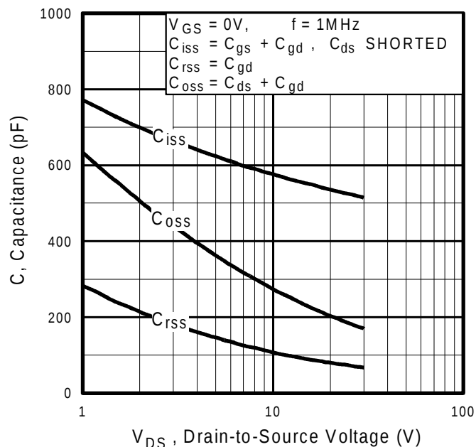
Fig 8. Typical Capacitance Vs. Drain-to-Source Voltage
