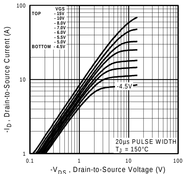
Fig 12. Typical Output Characteristics
