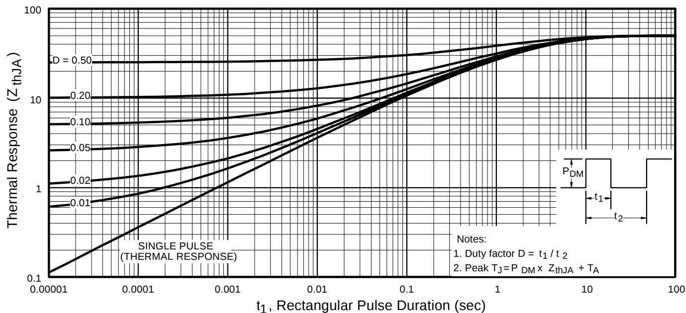
Fig 10. Maximum Effective Transient Thermal Impedance, Junction-to-Ambient
