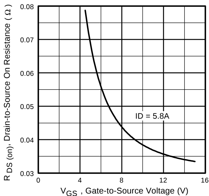
Fig 7. Typical On-Resistance Vs. Gate Voltage
