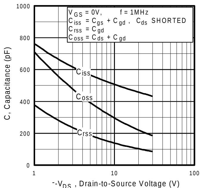
Fig 18. Typical Capacitance Vs. Drain-to-Source Voltage
