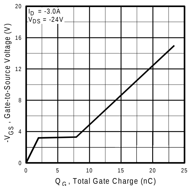
Fig 19. Typical Gate Charge Vs. Gate-to-Source Voltage
