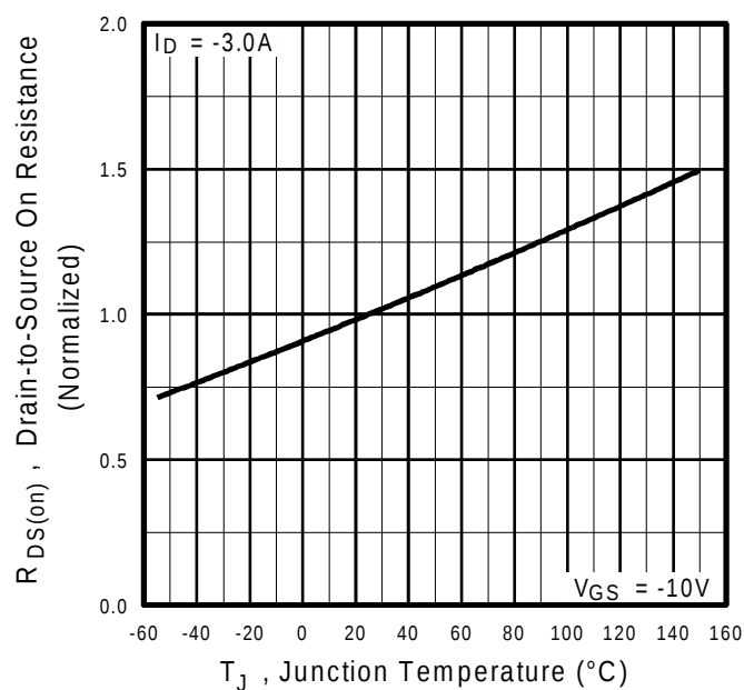
Fig 15. Normalized On-Resistance Vs. Temperature
