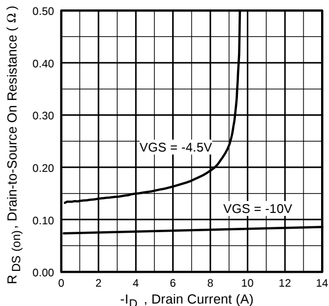
Fig 16. Typical On-Resistance Vs. Drain Current
