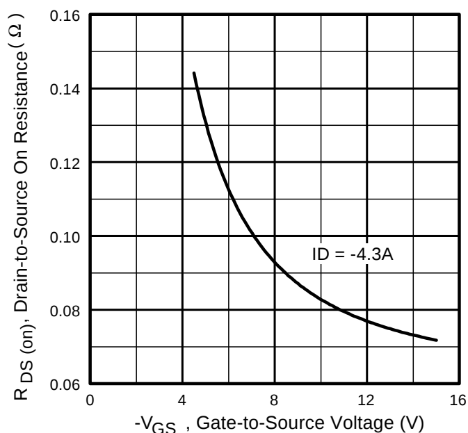
Fig 17. Typical On-Resistance Vs. Gate Voltage
