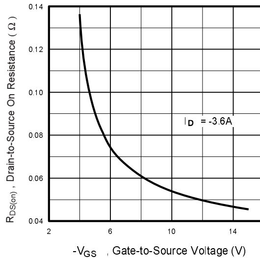
Fig 7. Typical On-Resistance Vs. Gate Voltage
