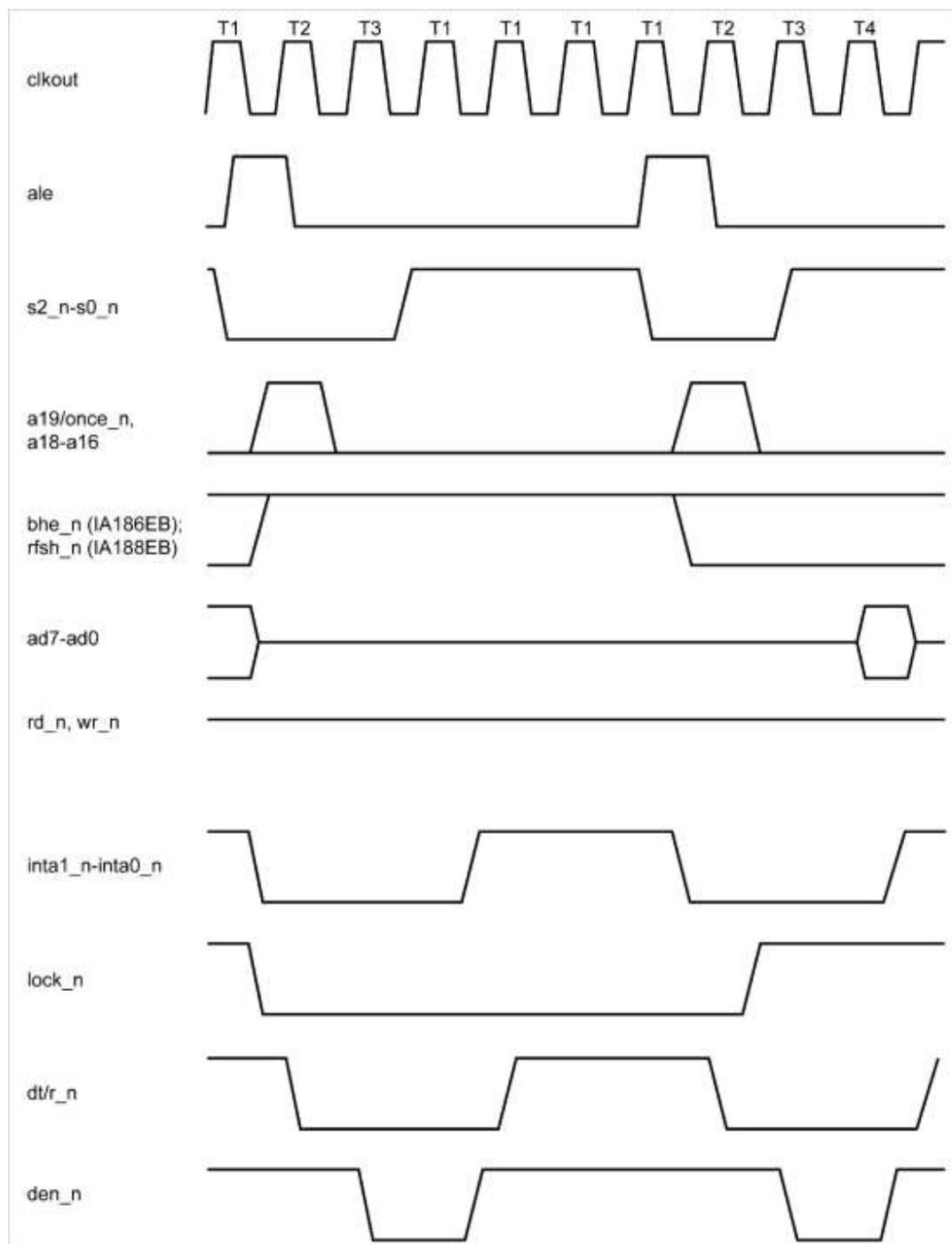
Figure 23. Interrupt Acknowledge (inta1_n, inta0_n) Cycle Timing
