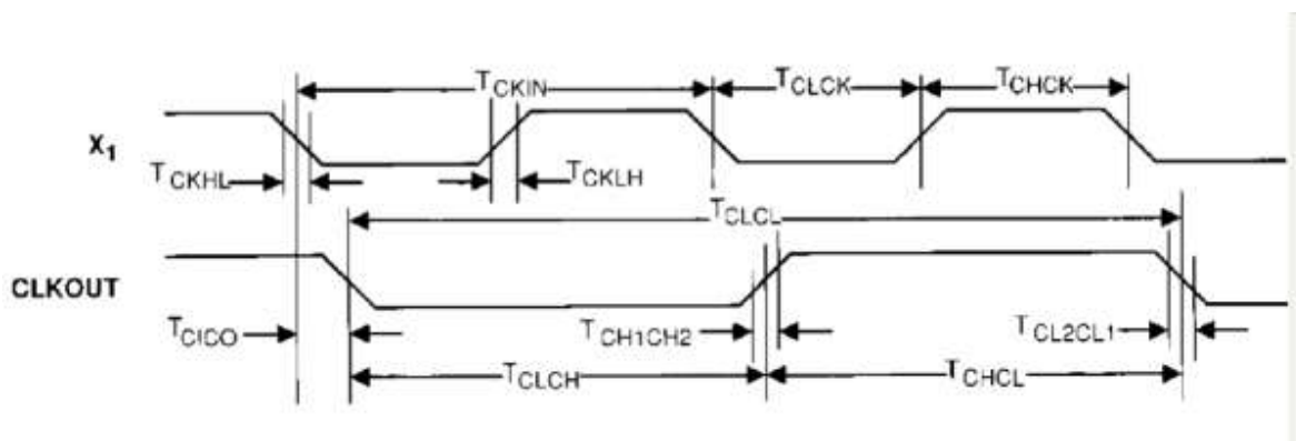
Figure 16. Clock Input and Clock Output Timing Characteristics
