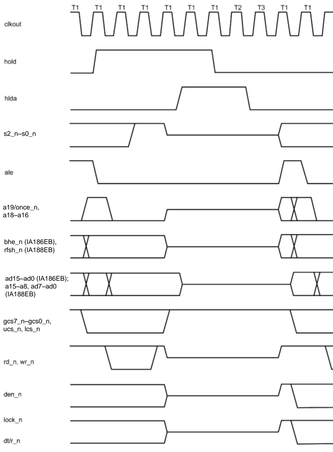
Figure 24. hold/hlda Timing
