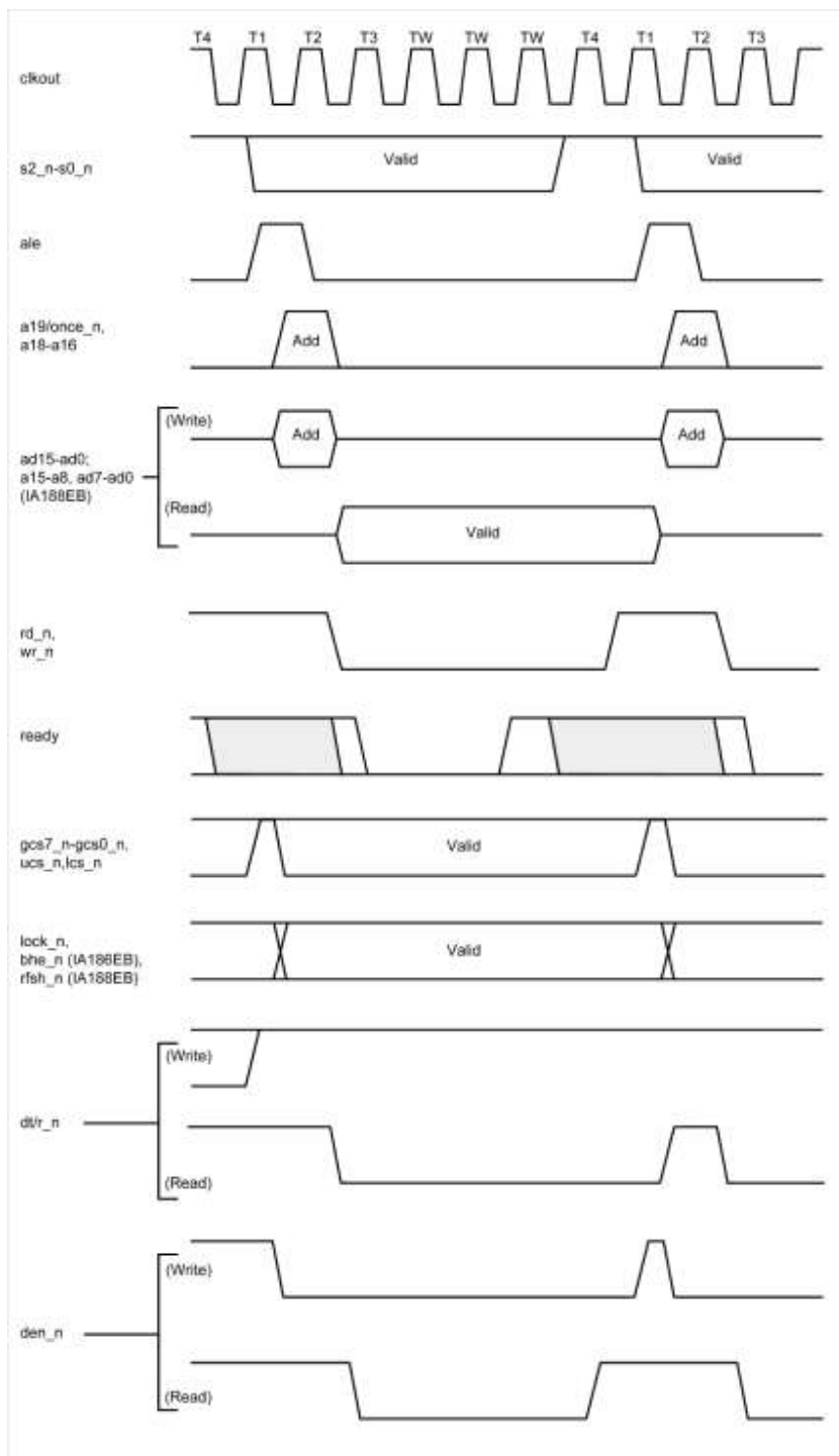
Figure 26. Ready Timing
