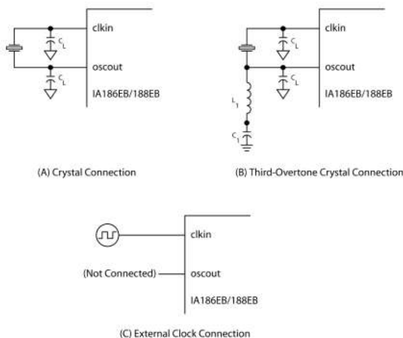
Figure 11. Clock Circuit Connection Options
