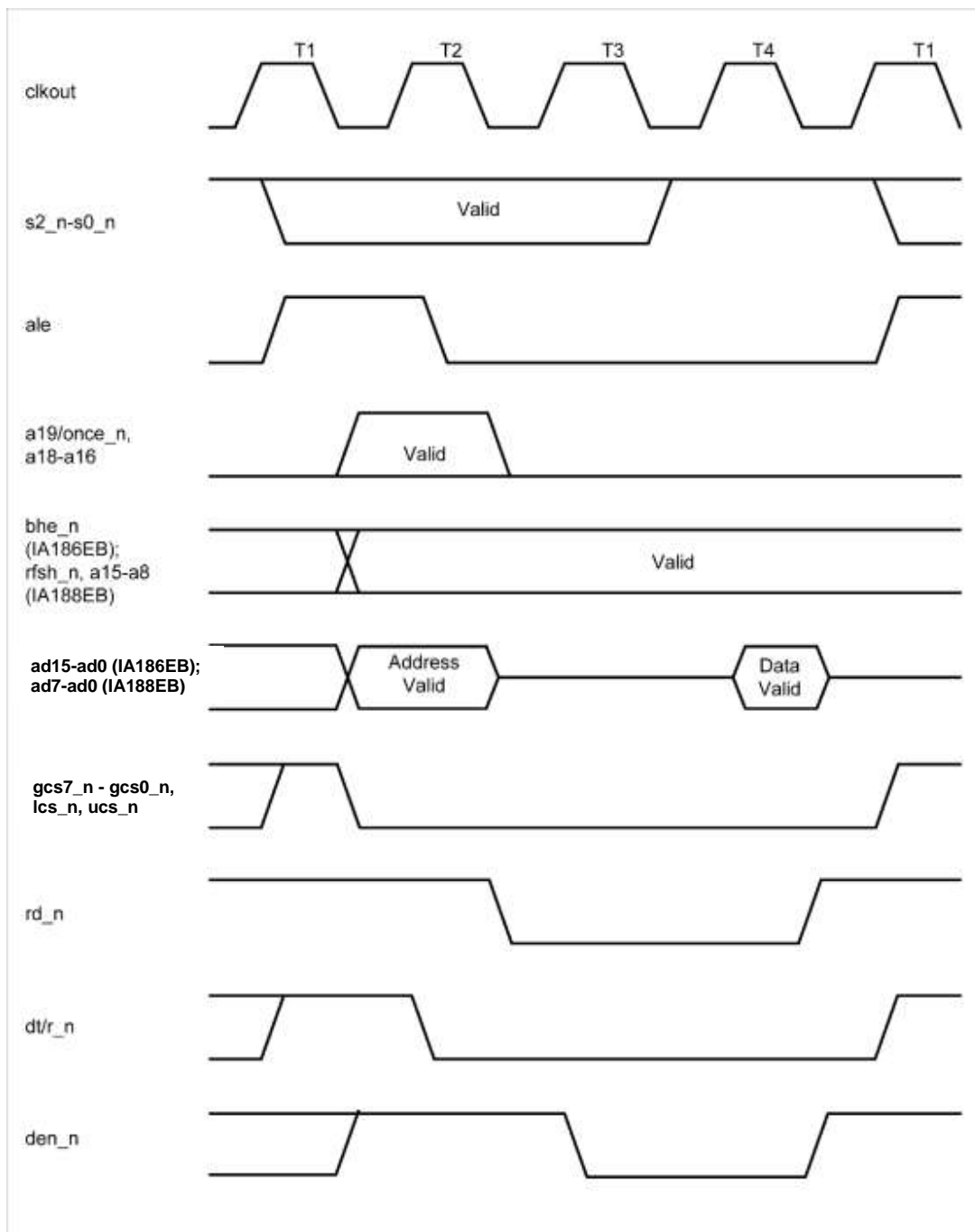
Figure 20. Read, Fetch, and Refresh Cycle Timing
