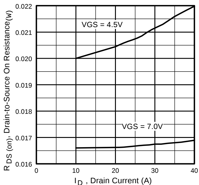
Fig 12. On-Resistance Vs. Drain Current
