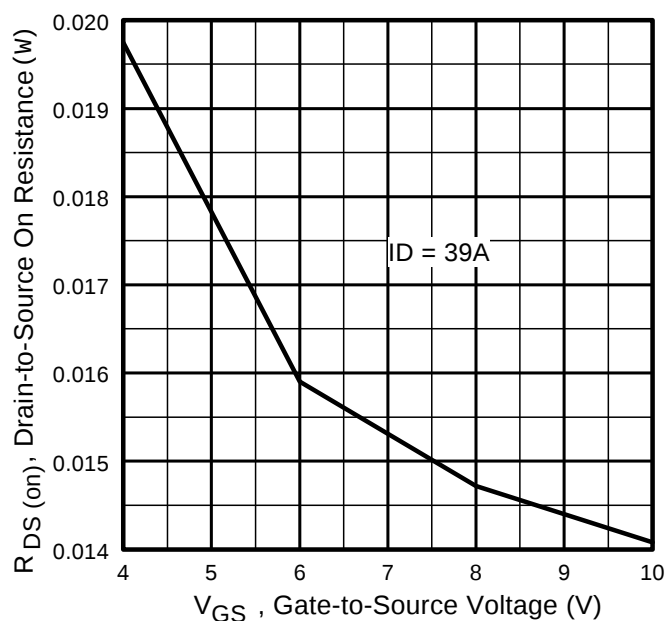
Fig 13. On-Resistance Vs. Gate Voltage
