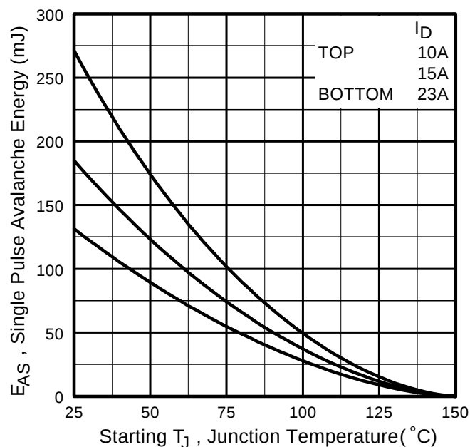
Fig 10. Maximum Avalanche Energy Vs. Drain Current
