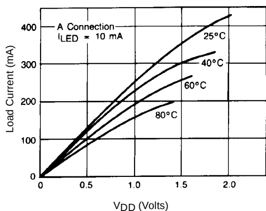
Figure 3. Typical On Characteristics (A Connection)
