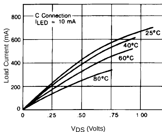
Figure 4. Typical On-Characteristics (C Connection)
