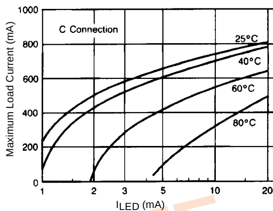
Figure 6. Typical Control Current Requirement (C Connection)
