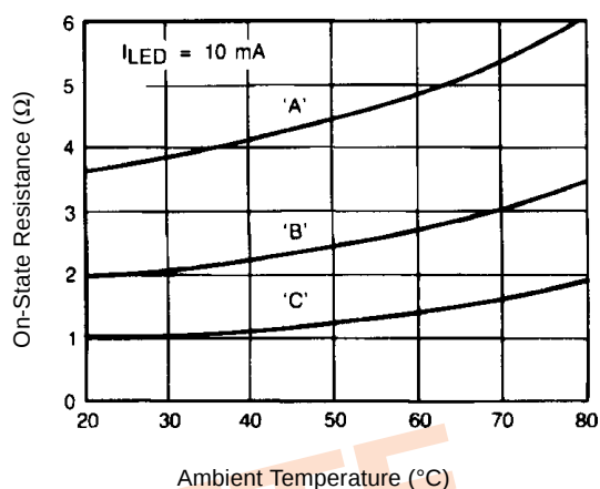
Figure 2. Typical On-Resistance
