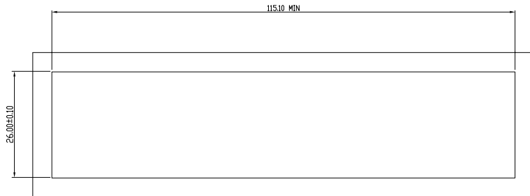
BEZEL CUT-OUT CENTER SPACING DETAIL BEZEL THICKNESS:0.8-2.6
