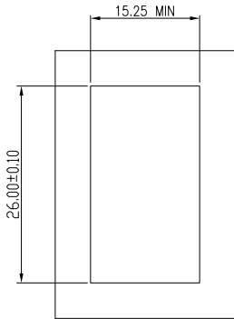
BEZEL CUT-OUT CENTER SPACING DETAIL BEZEL THICKNESS:0.8-2.6
