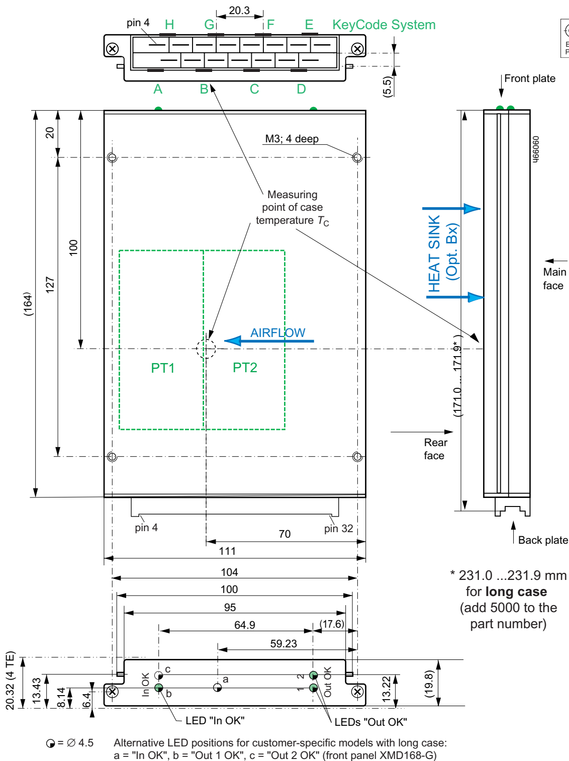
Fig. 23 Case Q04, weight approx. 500 g Aluminum, fully enclosed, black anodized and self cooling
