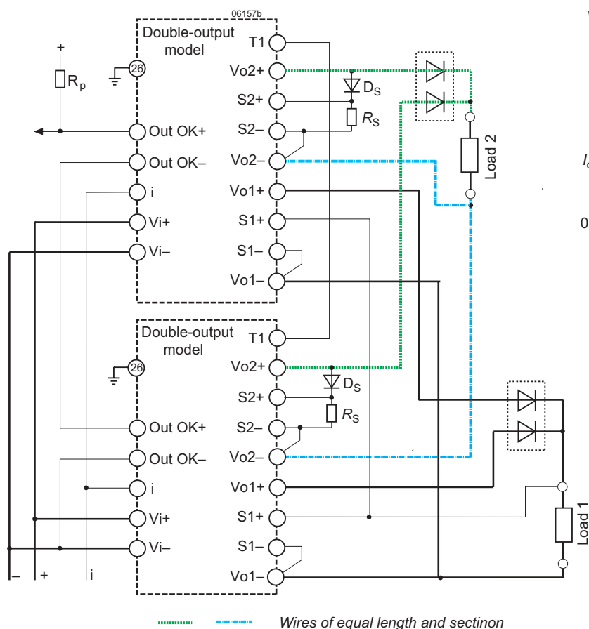
Fig. 11 Redundant configuration
