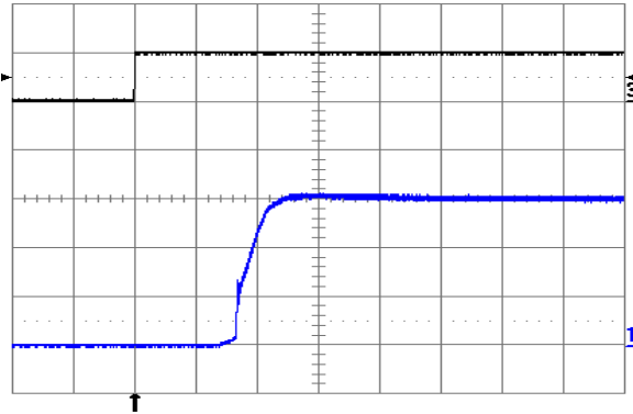
Fig. 1.5V.3: Turn-on transient at full rated load current (resistive) with no output capacitor at V_{in} = 48\text{ V} , triggered via ON/OFF pin. Top trace: ON/OFF signal (5 V/div.). Bottom trace: output voltage (0.5 V/div.). Time scale: 1 ms/div.
