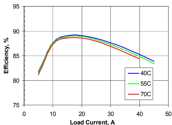
Figure 3. Efficiency vs. load current and ambient temperature for SQE48T50012 converter mounted vertically with V_{in}=48\text{V} and air flowing from pin 3 to pin 1 at 200LFM (1.0m/s).
