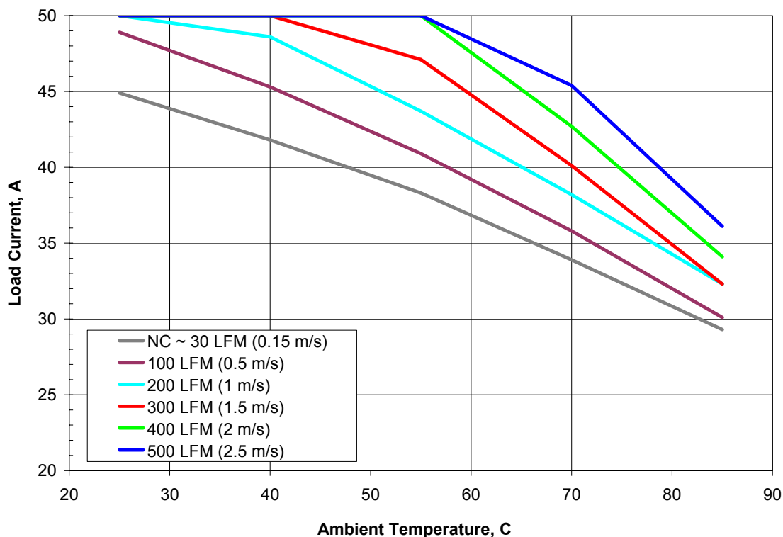
Figure 1. Available load current vs. ambient air temperature and airflow rates for SQE48T50012 converter mounted vertically with air flowing from pin 3 to pin 1, MOSFET temperature \leq 120^{\circ}\text{C} , V_{in} = 48\text{ V} .
