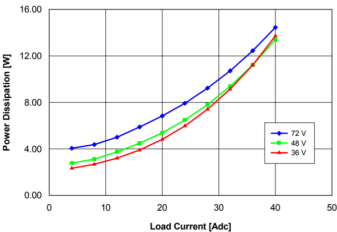
Fig. 3.3V.5: Power dissipation vs. load current and input voltage for converter mounted vertically with air flowing from pin 3 to pin 1 at a rate of 300 LFM (1.5 m/s) and Ta = 25 °C.
