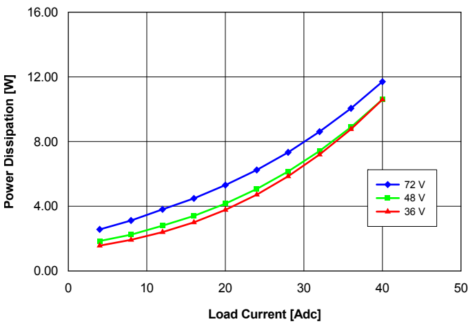
Fig. 1.8V.5: Power dissipation vs. load current and input voltage for converter mounted vertically with air flowing from pin 3 to pin 1 at a rate of 300 LFM (1.5 m/s) and Ta = 25 °C.
