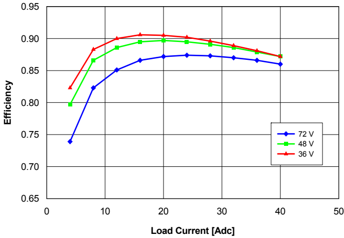
Fig. 1.8V.3: Efficiency vs. load current and input voltage for converter mounted vertically with air flowing from pin 3 to pin 1 at a rate of 300 LFM (1.5 m/s) and Ta = 25 °C.
