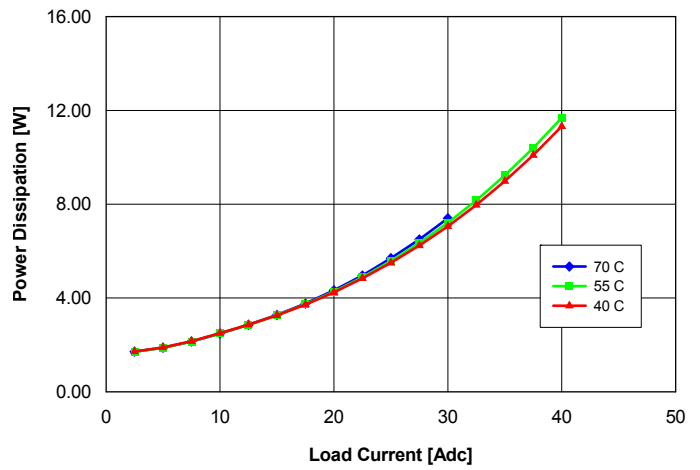
Fig. 1.8V.6: Power dissipation vs. load current and ambient temperature for converter mounted vertically with Vin = 48 V and air flowing from pin 3 to pin 1 at a rate of 200 LFM (1.0 m/s).
