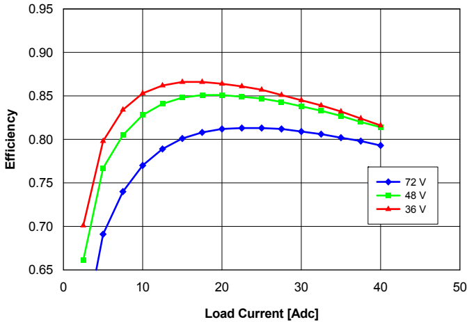
Fig. 1.0V.3: Efficiency vs. load current and input voltage for converter mounted vertically with air flowing from pin 3 to pin 1 at a rate of 300 LFM (1.5 m/s) and Ta = 25 °C.
