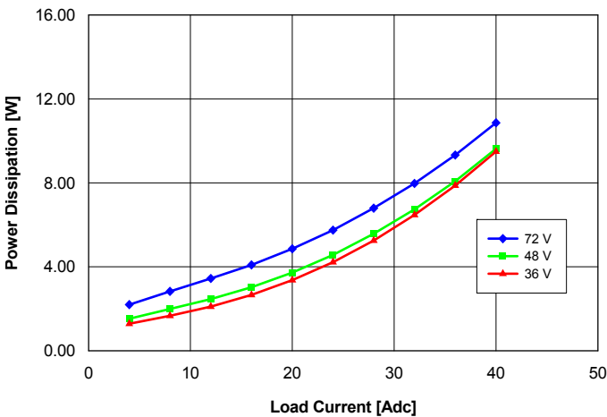
Fig. 1.2V.5: Power dissipation vs. load current and input voltage for converter mounted vertically with air flowing from pin 3 to pin 1 at a rate of 300 LFM (1.5 m/s) and Ta = 25 °C.
