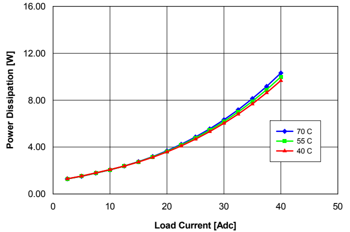
Fig. 1.0V.6: Power dissipation vs. load current and ambient temperature for converter mounted vertically with Vin = 48 V and air flowing from pin 3 to pin 1 at a rate of 200 LFM (1.0 m/s).
