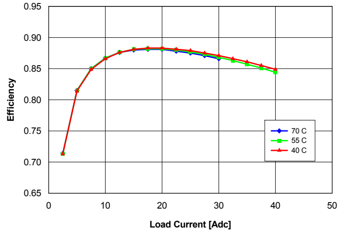
Fig. 1.5V.4: Efficiency vs. load current and ambient temperature for converter mounted vertically with Vin = 48 V and air flowing from pin 3 to pin 1 at a rate of 200 LFM (1.0 m/s).
