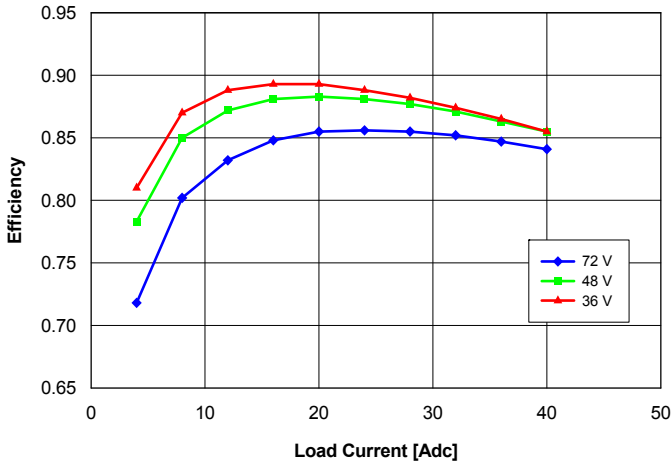
Fig. 1.5V.3: Efficiency vs. load current and input voltage for converter mounted vertically with air flowing from pin 3 to pin 1 at a rate of 300 LFM (1.5 m/s) and Ta = 25 °C.
