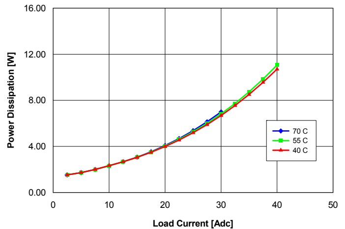
Fig. 1.5V.6: Power dissipation vs. load current and ambient temperature for converter mounted vertically with Vin = 48 V and air flowing from pin 3 to pin 1 at a rate of 200 LFM (1.0 m/s).
