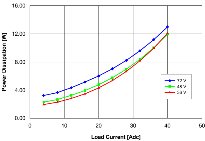
Fig. 2.5V.5: Power dissipation vs. load current and input voltage for converter mounted vertically with air flowing from pin 3 to pin 1 at a rate of 300 LFM (1.5 m/s) and Ta = 25 °C.
