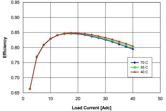
Fig. 1.0V.4: Efficiency vs. load current and ambient temperature for converter mounted vertically with Vin = 48 V and air flowing from pin 3 to pin 1 at a rate of 200 LFM (1.0 m/s).
