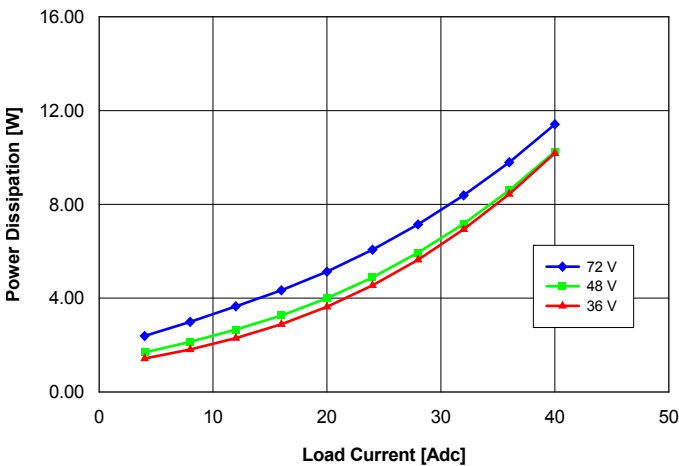
Fig. 1.5V.5: Power dissipation vs. load current and input voltage for converter mounted vertically with air flowing from pin 3 to pin 1 at a rate of 300 LFM (1.5 m/s) and Ta = 25 °C.
