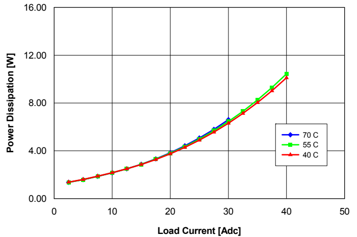
Fig. 1.2V.6: Power dissipation vs. load current and ambient temperature for converter mounted vertically with Vin = 48 V and air flowing from pin 3 to pin 1 at a rate of 200 LFM (1.0 m/s).
