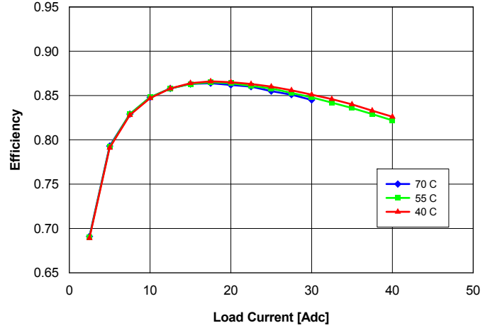
Fig. 1.2V.4: Efficiency vs. load current and ambient temperature for converter mounted vertically with Vin = 48 V and air flowing from pin 3 to pin 1 at a rate of 200 LFM (1.0 m/s).
