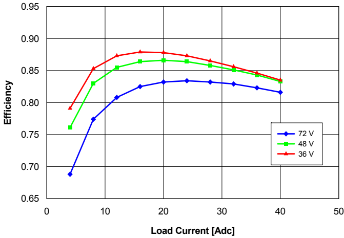
Fig. 1.2V.3: Efficiency vs. load current and input voltage for converter mounted vertically with air flowing from pin 3 to pin 1 at a rate of 300 LFM (1.5 m/s) and Ta = 25 °C.
