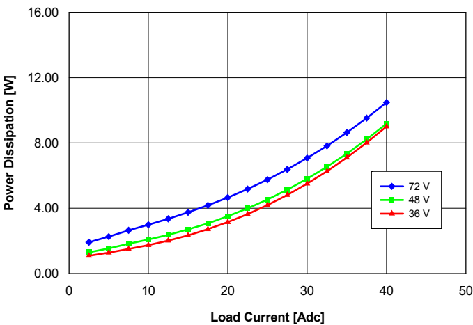
Fig. 1.0V.5: Power dissipation vs. load current and input voltage for converter mounted vertically with air flowing from pin 3 to pin 1 at a rate of 300 LFM (1.5 m/s) and Ta = 25 °C.
