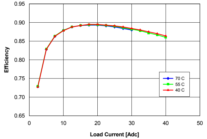
Fig. 1.8V.4: Efficiency vs. load current and ambient temperature for converter mounted vertically with Vin = 48 V and air flowing from pin 3 to pin 1 at a rate of 200 LFM (1.0 m/s).
