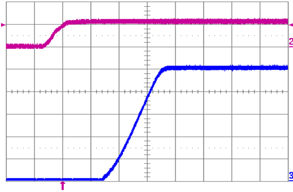
Fig. 5.0V.5: Turn-on transient (YNL12S10050) with application of V_{in} at full rated load current (resistive) and 100\ \mu\text{F} external capacitance at V_{in} = 12\ \text{V} . Top trace: V_{in} (10 V/div.); Bottom trace: output voltage (1 V/div.); Time scale: 2 ms/div.
