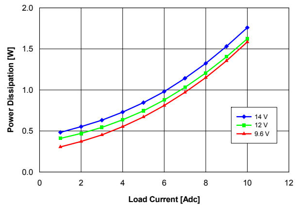
Fig. 1.0V.4: Power loss vs. load current and input voltage for YNL12S10010 converter mounted vertically with air flowing at a rate of 200 LFM (1 m/s) and T_a = 25\text{ }^{\circ}\text{C} .
