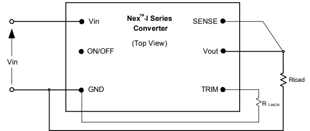
Fig. C: Configuration for increasing output voltage.
