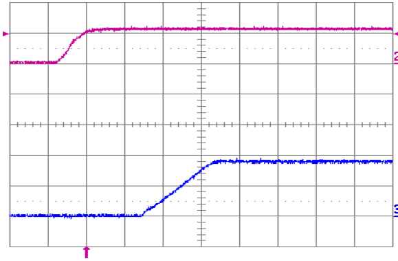
Fig. 1.8V.5: Turn-on transient (YNL12S10018) with application of V_{in} at full rated load current (resistive) and 100\ \mu\text{F} external capacitance at V_{in} = 12\ \text{V} . Top trace: V_{in} (10 V/div.); Bottom trace: output voltage (1 V/div.); Time scale: 2 ms/div.
