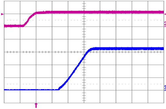
Fig. 3.3V.5: Turn-on transient (YNL12S10033) with application of V_{in} at full rated load current (resistive) and 100\ \mu\text{F} external capacitance at V_{in} = 12\ \text{V} . Top trace: V_{in} (10 V/div.); Bottom trace: output voltage (1 V/div.); Time scale: 2 ms/div.
