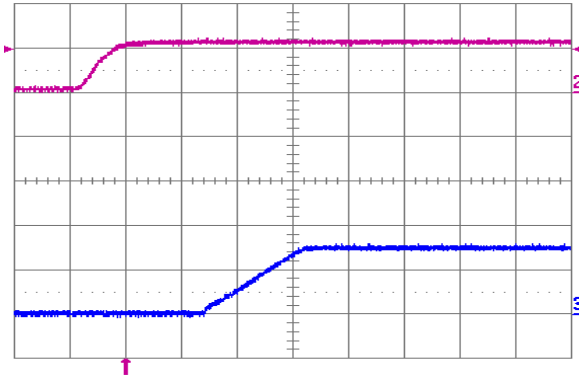
Fig. 1.5V.5: Turn-on transient (YNL12S10015) with application of V_{in} at full rated load current (resistive) and 100 \mu\text{F} external capacitance at V_{in} = 12\text{ V} . Top trace: V_{in} (10 V/div.); Bottom trace: output voltage (1 V/div.); Time scale: 2 ms/div.
