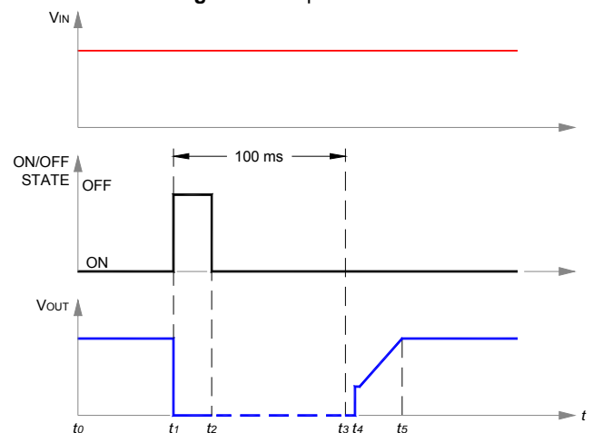
Fig. 9: Start-up scenario #3.
