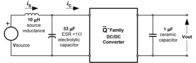
Fig. 23: Test setup for measuring input reflected ripple currents, i_c and i_s .
