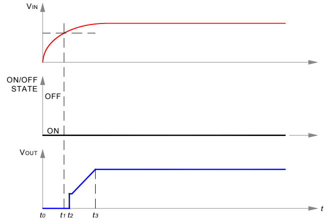
Fig. 7: Start-up scenario #1.
