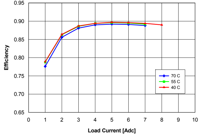
Fig. 15: Efficiency vs. load current and ambient temperature for converter mounted vertically with Vin = 54 V and air flowing from pin 3 to pin 1 at a rate of 200 LFM (1.0 m/s).
