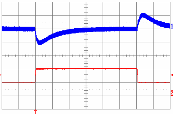
Fig. 20: Output voltage response to load current step-change (2 A – 4 A – 2 A) at V_{in} = 48\text{ V} . Top trace: output voltage (200 mV/div). Bottom trace: load current (2 A/div.). Current slew rate: 0.1 A/ \mu\text{s} . C_o = 1\ \mu\text{F} ceramic. Time scale: 0.5 ms/div.
