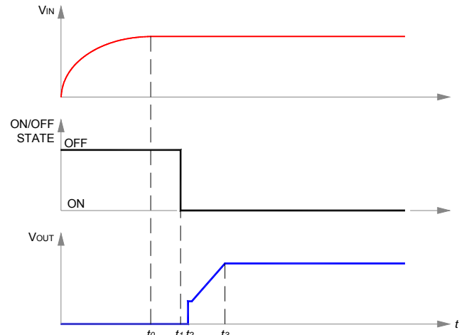
Fig. 8: Start-up scenario #2.
