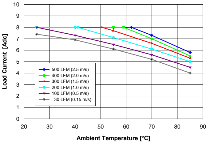
Fig. 1: Available load current vs. ambient air temperature and air-flow rates for Q48S08120 converter mounted vertically with air flowing from pin 3 to pin 1, MOSFET temperature \leq 120^{\circ}\text{C} , V_{in} = 54\text{ V} .
