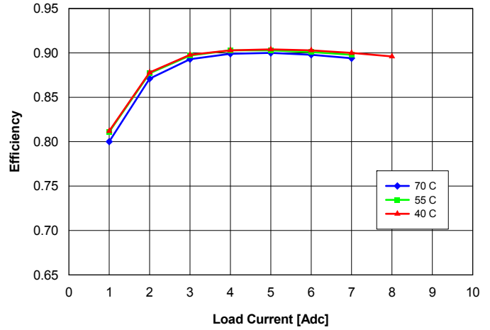
Fig. 17: Efficiency vs. load current and ambient temperature for converter mounted horizontally with Vin = 54 V and air flowing from pin 3 to pin 4 at a rate of 200 LFM (1.0 m/s).
