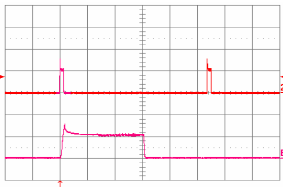
Fig. 27: Load current (top trace, 10 A/div, 20 ms/div) into a 10 mΩ short circuit during restart, at V_{in} = 48 V. Bottom trace (10 A/div, 1 ms/div) is an expansion of the on-time portion of the top trace.
