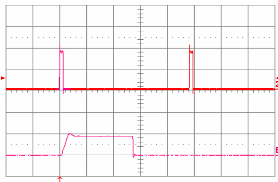
Fig. 27: Load current (top trace, 20 A/div, 20 ms/div) into a 10 mΩ short circuit during restart, at Vin = 48 V. Bottom trace (40 A/div, 1 ms/div) is an expansion of the on-time portion of the top trace.
