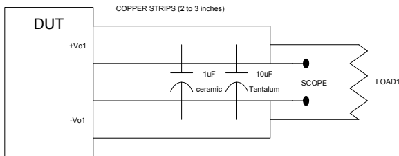
Figure 9. Output Ripple and Noise Measurement Test Setup
