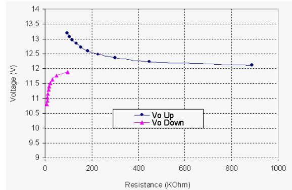
Figure 14. Trim Value Characteristic.
