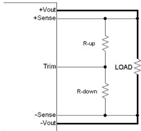
Figure 15. Converter Trim Schematic
