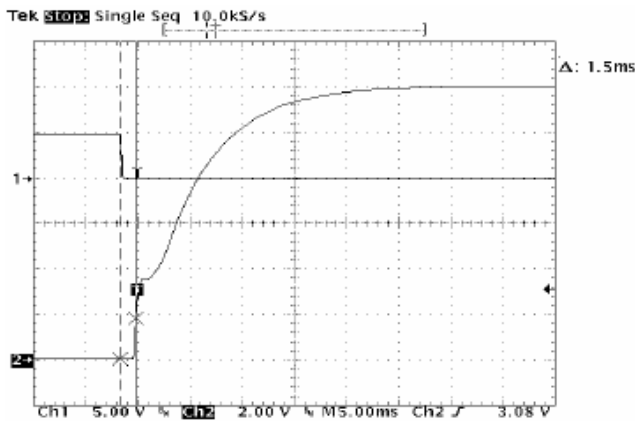
Figure 6. Turn-On Characteristics via On/Off Ctrl (typ)
