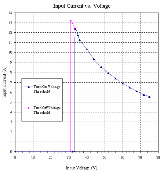
Figure 2. Undervoltage Lockout Characteristics (typ)
