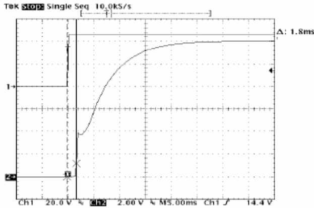
Figure 5. Turn-On Characteristics @ Power-up (typ)
