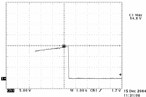
Figure 13. Induced OVP Behavior (typ).
