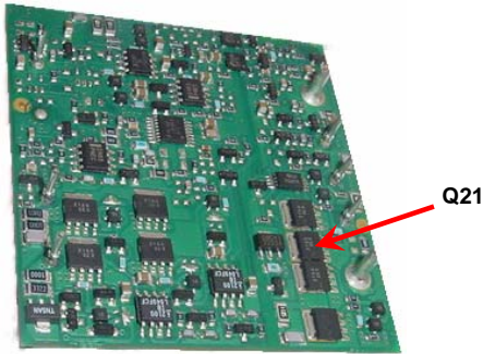
Figure 18. Thermal Reference Q21 (I/O pin side)
