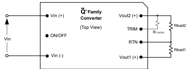
Fig. 4: Configuration for decreasing output voltage.
