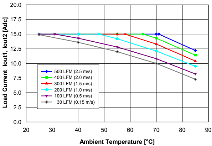
Fig. 10: Available balanced load current ( I_{out1} = I_{out2} ) vs. ambient air temperature and airflow rates for converter mounted vertically with V_{in} = 48\text{ V} , air flowing from pin 3 to pin 1 and maximum FET temperature \leq 120^\circ\text{C} .
