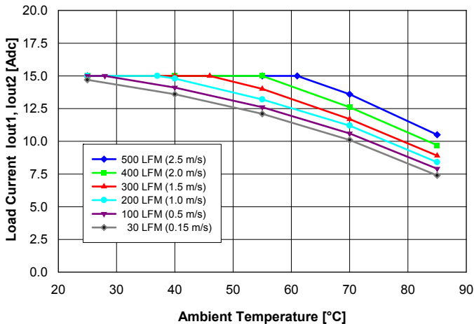
Fig. 14: Available balanced load current (Iout1 = Iout2) vs. ambient air temperature and airflow rates for converter mounted vertically with Vin = 48 V, air flowing from pin 3 to pin 4 and maximum FET temperature ≤ 120°C.
