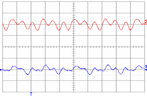
Fig. 34: Output voltage ripple at full rated load current into a resistive load on both outputs with C_o = 1\mu\text{F} (ceramic) and V_{in} = 48\text{ V} . Ch2 = V_{out2} , Ch1 = V_{out1} (both 20 mV/div). Time scale: 1\mu\text{s/div} .
