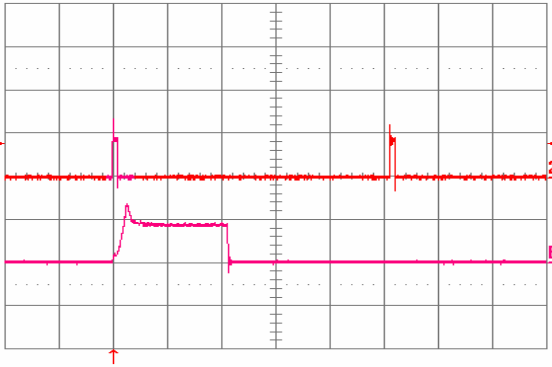
Fig. 32: Load current i_{out1} into a 10\text{ m}\Omega short circuit on V_{out1} during restart, with V_{out2} open (no load), at V_{in} = 48\text{ V} . Ch2 = i_{out1} (20 A/div, 20 ms/div). ChB = i_{out1} (20 A/div, 1 ms/div) is an expansion of the on-time portion of i_{out1} .
