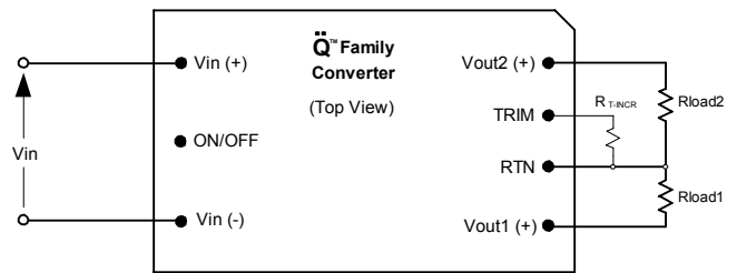
Fig. 3: Configuration for increasing output voltage.
