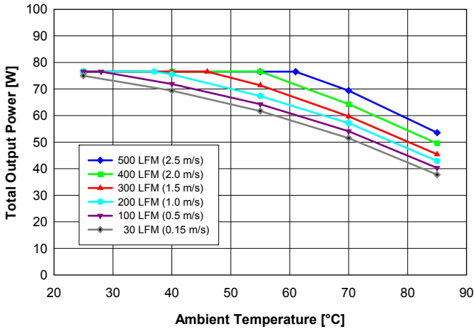
Fig. 12: Available output power for balanced load current (Iout1 = Iout2) vs. ambient air temperature and airflow rates for converter mounted vertically with Vin = 48 V, air flowing from pin 3 to pin 4 and maximum FET temperature ≤ 120°C.
