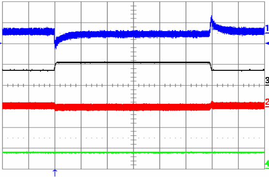
Fig. 24: Output voltage response to lout1 load current step-change of 3.75 A (50%-75%-50%) at lout2 = 7.5 A and Vin = 48 V. Ch1 = Vout1 (50 mV/div), Ch2 = Vout2 (50 mV/div), Ch3 = lout1 (10 A/div.), Ch4 = lout2 (10 A/div.). Current slew rate: 0.1 A/ \mu s, Co = 10 \mu F tantalum + 1 \mu F ceramic. Time scale: 0.5 ms/div.
