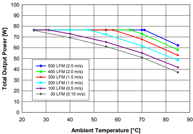
Fig. 1: Available output power vs. ambient air temperature and airflow rates for QD48S018033 converter mounted vertically with air flowing from pin 3 to pin 1, MOSFET temperature \leq 120^\circ\text{C} , V_{in} = 48\text{ V} and balanced load on both outputs ( I_{out1} = I_{out2} ).
