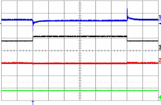
Fig. 26: Output voltage response to lout1 load current step-change of 3.75 A (50%-75%-50%) at lout2 = 7.5 A and Vin = 48 V. Ch1 = Vout1 (100 mV/div), Ch2 = Vout2 (100 mV/div), Ch3 = lout1 (10 A/div.), Ch4 = lout2 (10 A/div.). Current slew rate: 5 A/ \mu s, Co = 300 \mu F tantalum + 1 \mu F ceramic. Time scale: 0.5 ms/div.
