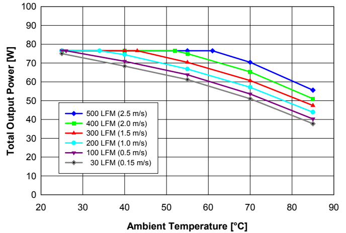
Fig. 13: Available output power for balanced load current (Iout1 = Iout2) vs. ambient air temperature and airflow rates for converter mounted vertically with Vin = 48 V, air flowing from pin 4 to pin 3 and maximum FET temperature ≤ 120°C.
