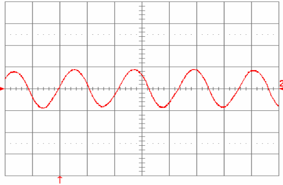
Fig. 36: Input reflected ripple current, i_c (100 mA/div), measured at input terminals at full rated load current on both outputs and V_{in} = 48 V. Refer to Fig. 35 for test setup. Time scale: 1 \mu s/div.
