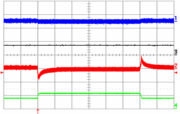
Fig. 25: Output voltage response to lout2 load current step-change of 3.75 A (50%-75%-50%) at lout1 = 7.5 A and Vin = 48 V. Ch1 = Vout1 (50 mV/div), Ch2 = Vout2 (50 mV/div), Ch3 = lout1 (10 A/div.), Ch4 = lout2 (10 A/div.). Current slew rate: 0.1 A/ \mu s, Co = 10 \mu F tantalum + 1 \mu F ceramic. Time scale: 0.5 ms/div.
