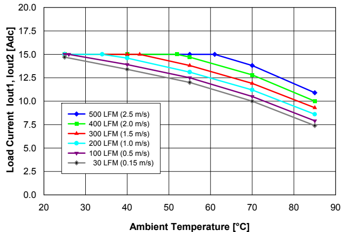
Fig. 15: Available balanced load current (Iout1 = Iout2) vs. ambient air temperature and airflow rates for converter mounted vertically with Vin = 48 V, air flowing from pin 4 to pin 3 and maximum FET temperature ≤ 120°C.
