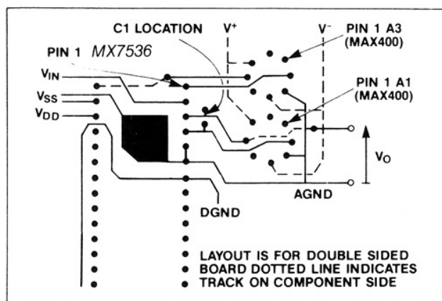
Figure 6. Suggested Layout for MX7536 Circuit of Figure 4
