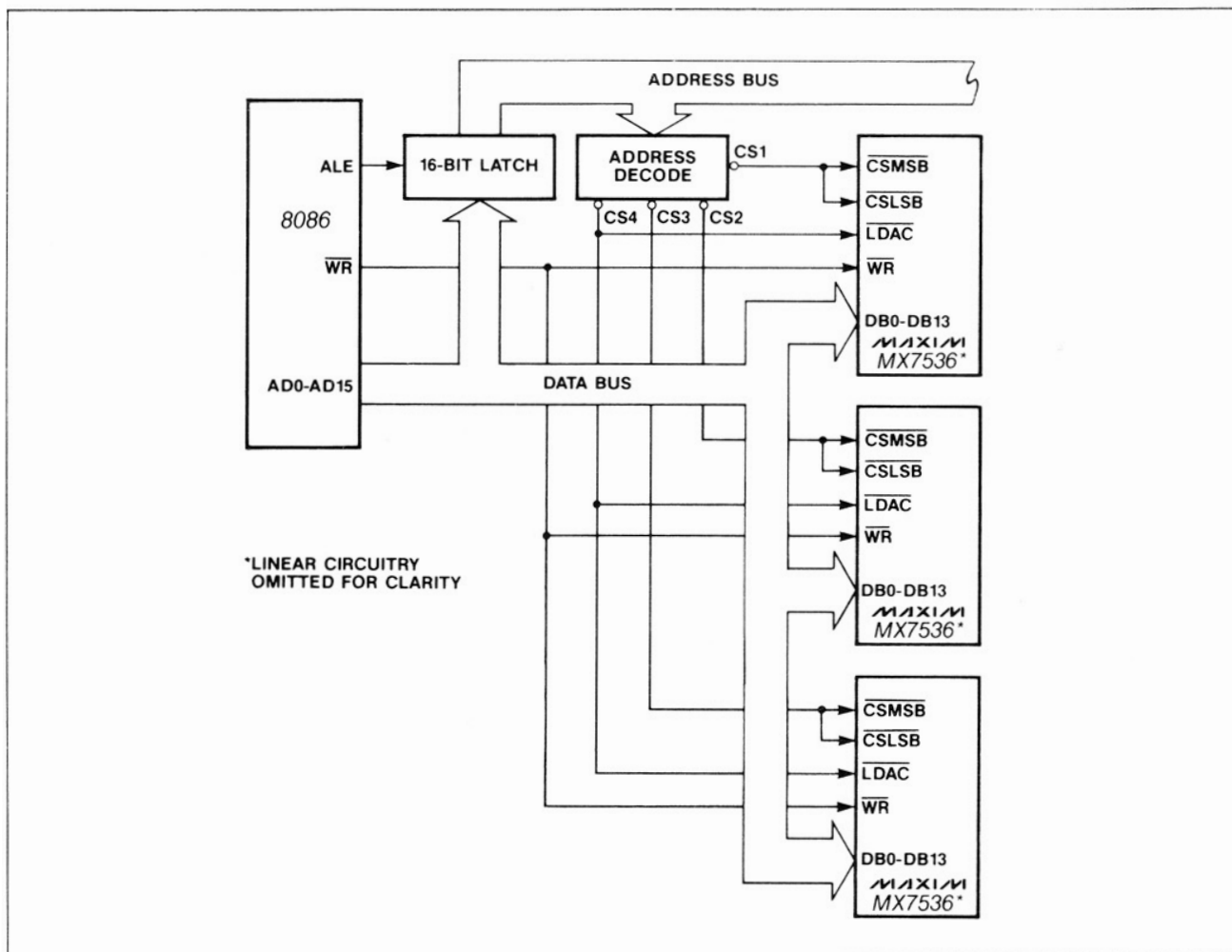
Figure 8. MX7536-8086 Interface: Multiple DAC System
