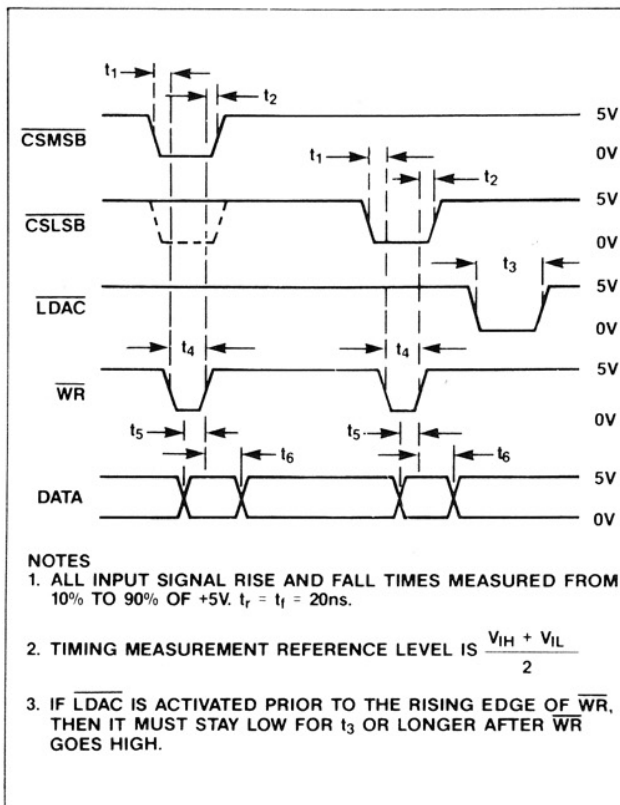
Figure 1. MX7536 Timing Diagram
