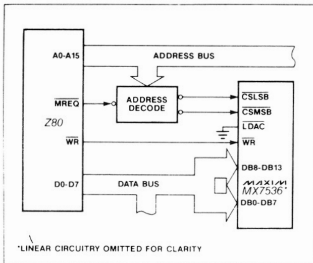
Figure 10. MX7536-Z80 Interface
