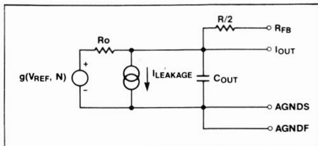
Figure 3. Equivalent Analog Output Circuit
