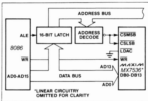
Figure 7. MX7536-8086 Interface Circuit
