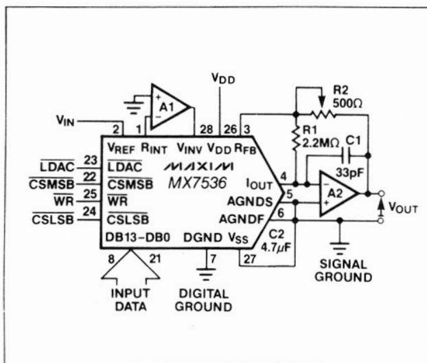
Figure 4. MX7536 Operation
