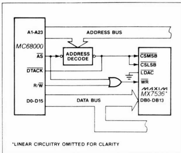
Figure 9. MX7536-MC68000 Interface
