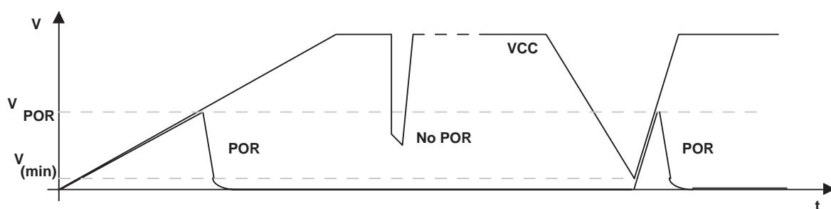
Figure 3. Power-On Reset (POR) vs Supply Voltage
