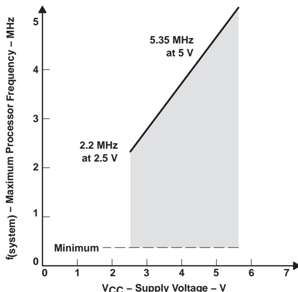
Figure 1. C Version Frequency vs Supply Voltage
