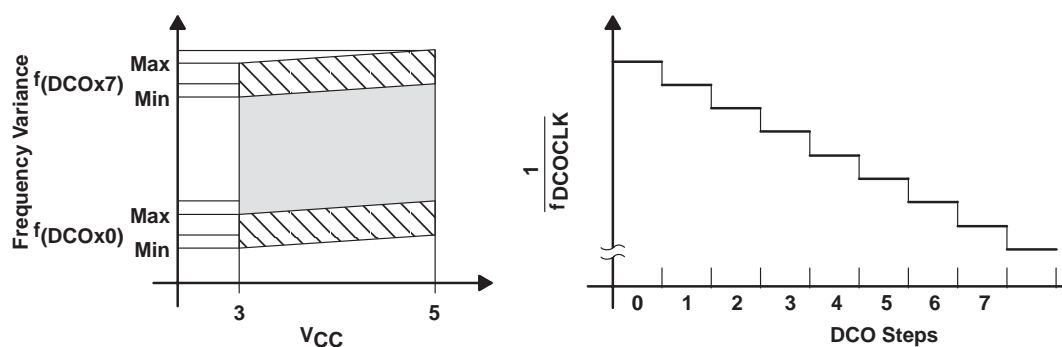
Figure 5. DCO Characteristics
