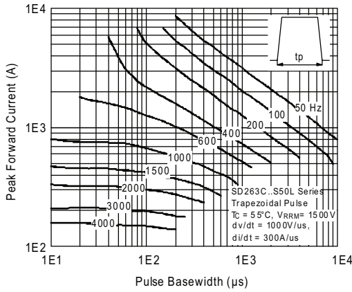
Fig. 18 - Frequency Characteristics
