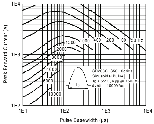
Fig. 16 - Frequency Characteristics
