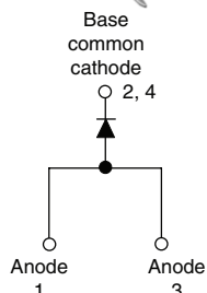
TO-247AC
