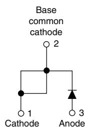
TO-247AC modified
