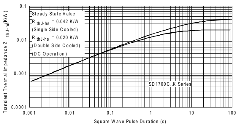
Fig. 19 - Thermal Impedance Z_{thJC} Characteristics
