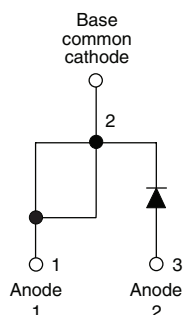
TO-247AC modified
