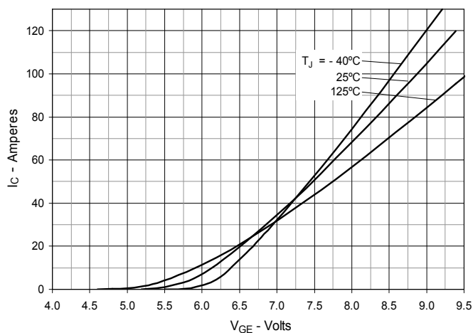
Fig. 6. Input Admittance
