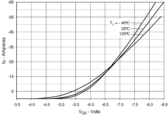
Fig. 7. Input Admittance
