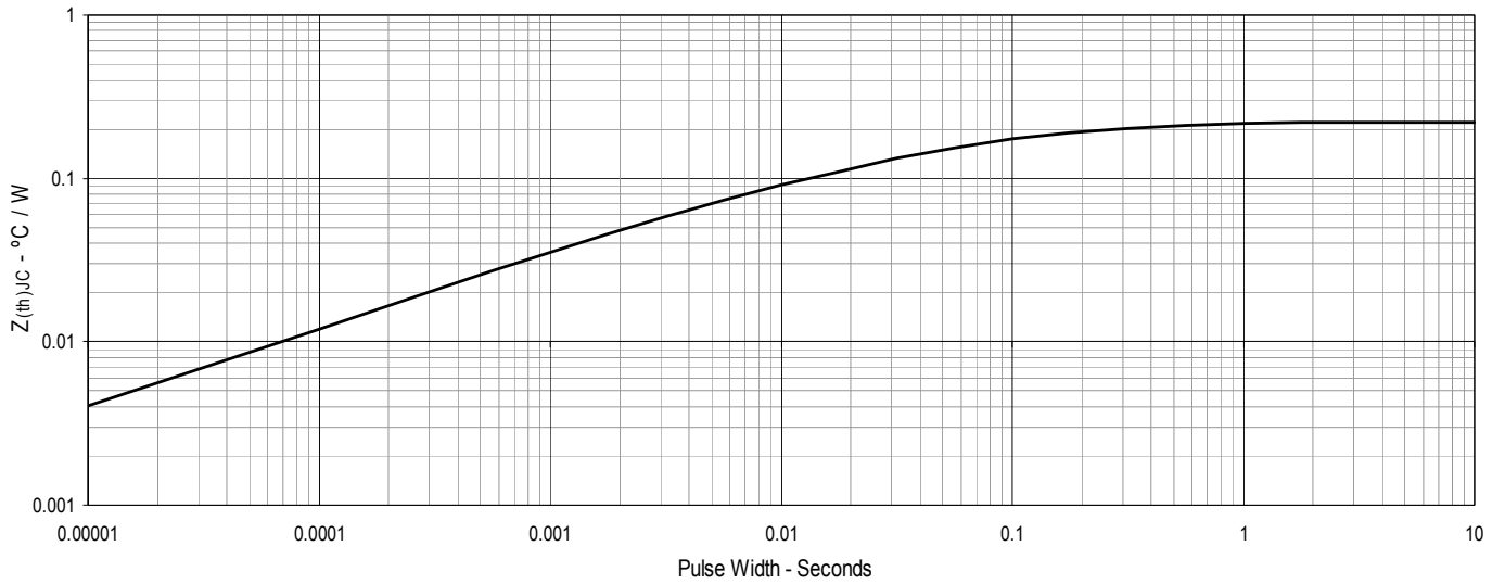
Fig. 19. Maximum Transient Thermal Impedance
