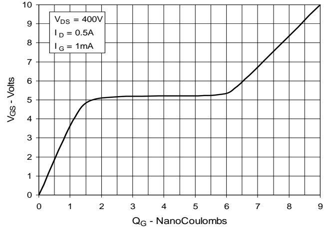
Fig. 10. Gate Charge
