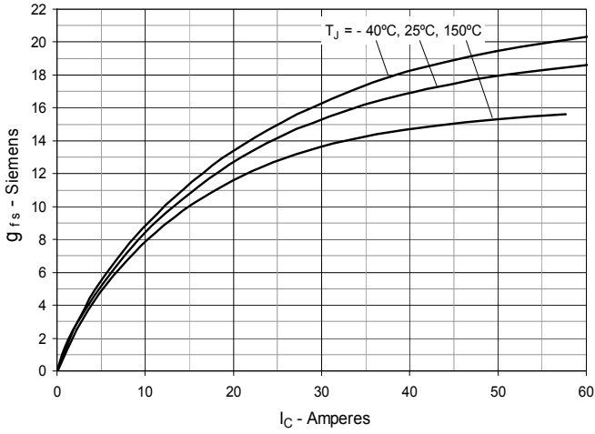
Fig. 7. Transconductance
