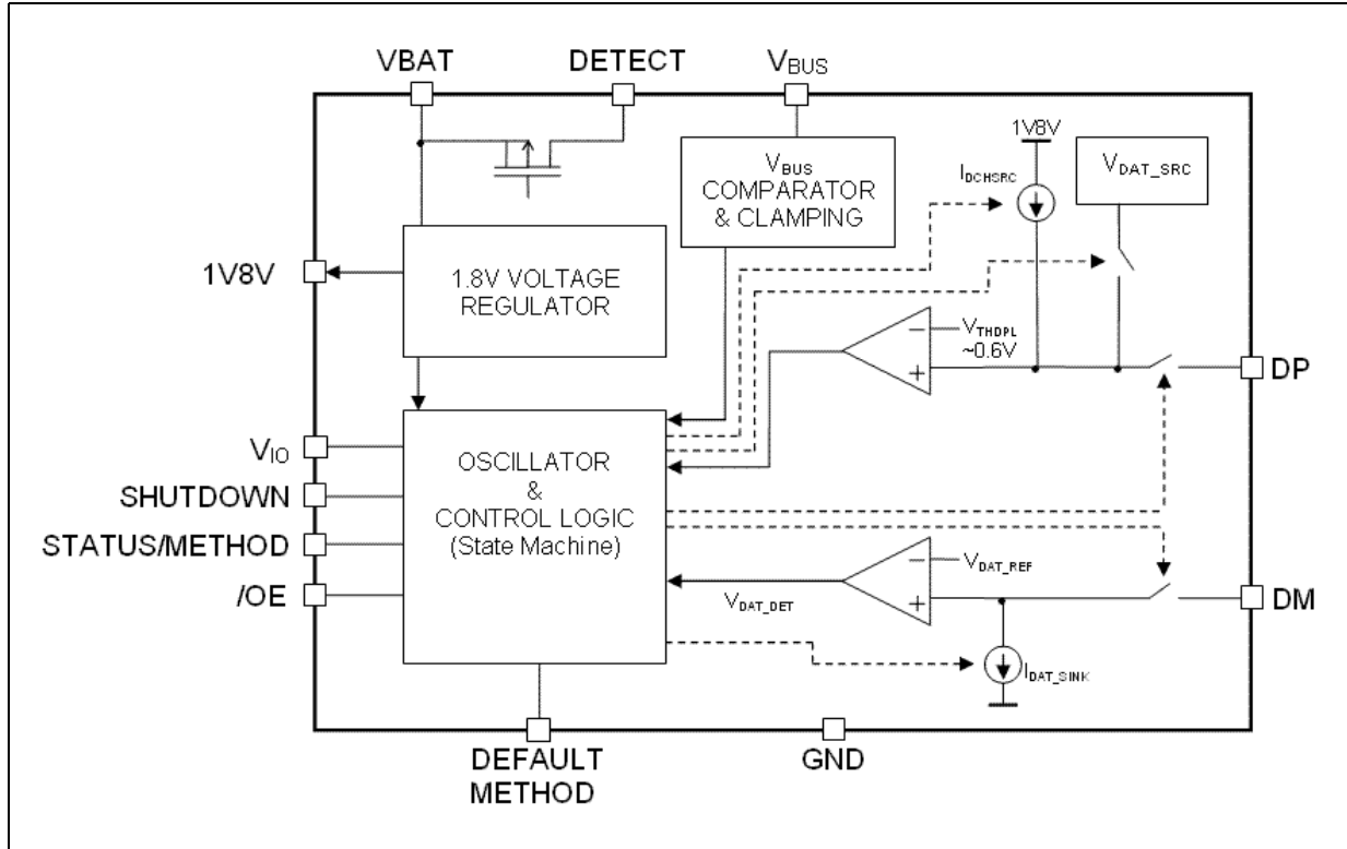
Figure 3. Functional diagram
