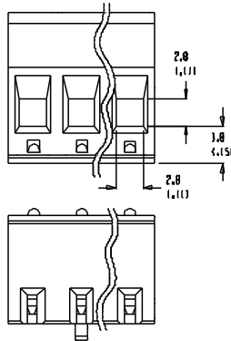
SECTION Z-Z
