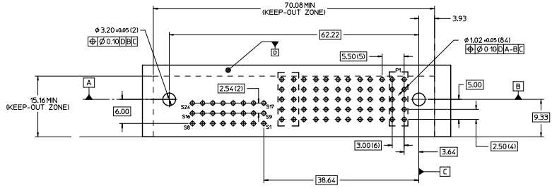
RECOMMENDED PC BOARD LAYOUT & KEEP-OUT ZONE
