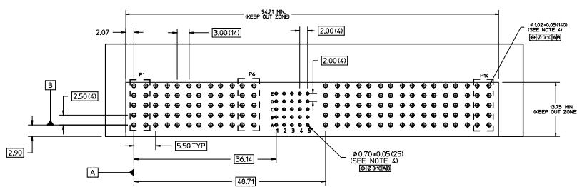
RECOMMENDED PCB LAYOUT AND KEEP-OUT ZONE
