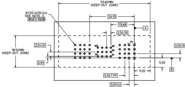
RECOMMENDED PCB LAYOUT AND KEEP-OUT ZONE
