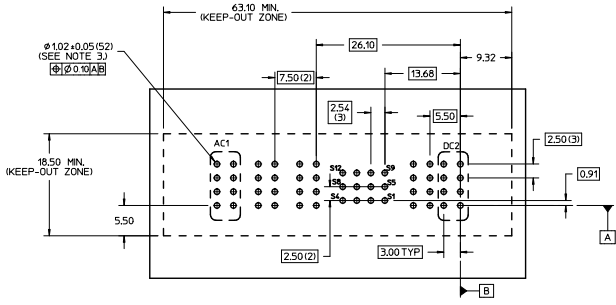
RECOMMENDED PCB LAYOUT AND KEEP-OUT ZONE
