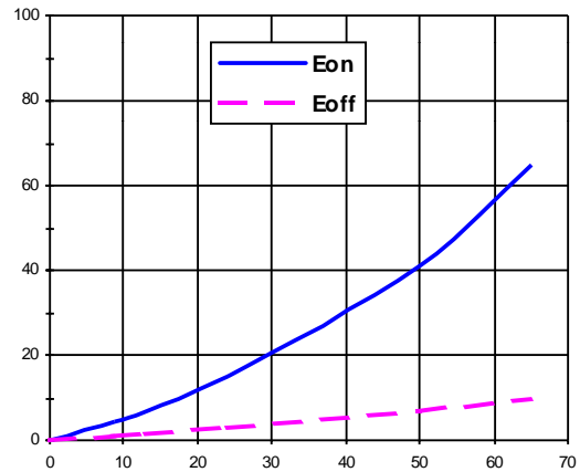
Figure 18 - E_{on} , E_{off} (mJ) Vs I_{out} (A)
