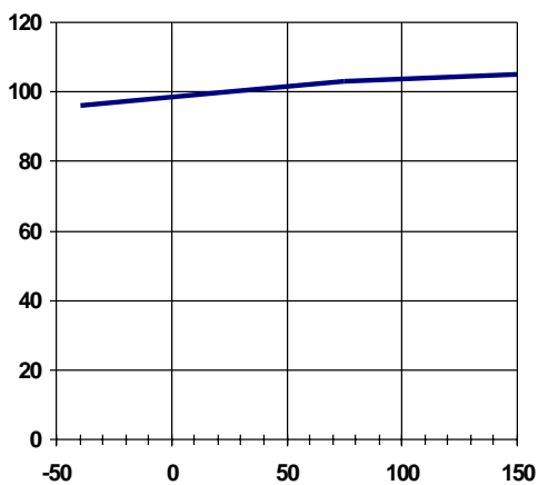
Figure 13 - I sd (A) Vs T j (°C)
