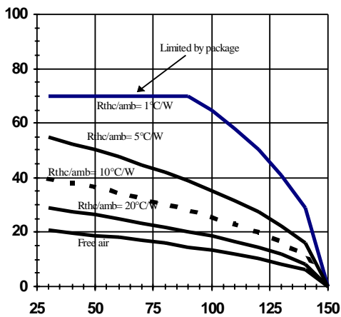
Figure 11 - Max. load current (A) Vs Temperature (°C)
