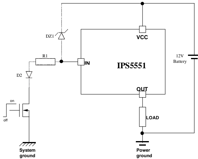
DZ1, R1 : optional additional voltage transient protection D2 : optional additional reverse battery protection See application note for details
