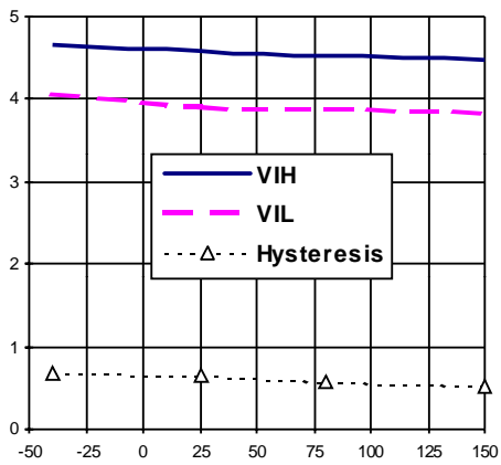
Figure 17 - V_{IH} , V_{IL} threshold (V) Vs T_j (°C)
