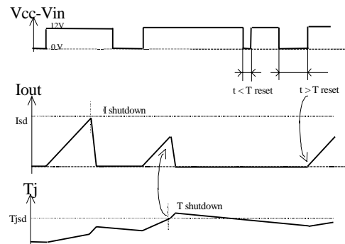
Figure 4 - Protection timing diagram
