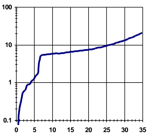
Figure 15 - I cc (mA) Vs V cc -V in (V)
