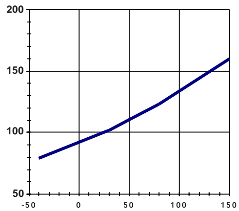
Figure 8 - Normalized Rds(on) (%) Vs T j (°C)
