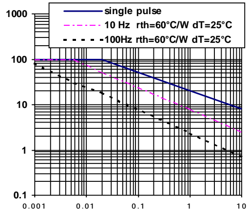
Figure 10 - Iclamp (A) Vs Inductive Load (μH)
