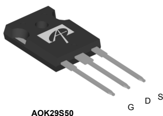
TO-247
