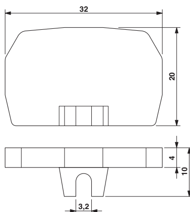
Dimensional drawing
