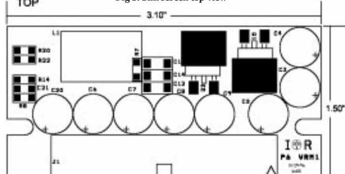
Fig 3. Silk screen top view
