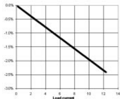
Fig 11. Load Regulation, 2.1 Volts Out
