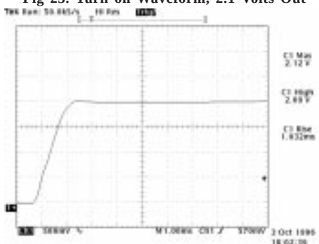
Fig 23. Turn on Waveform, 2.1 Volts Out
