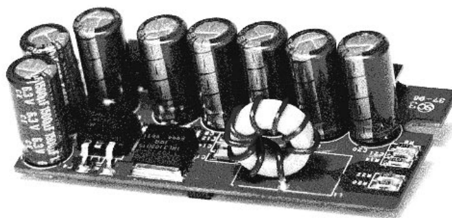
Figure 1. IRP6VRM1
