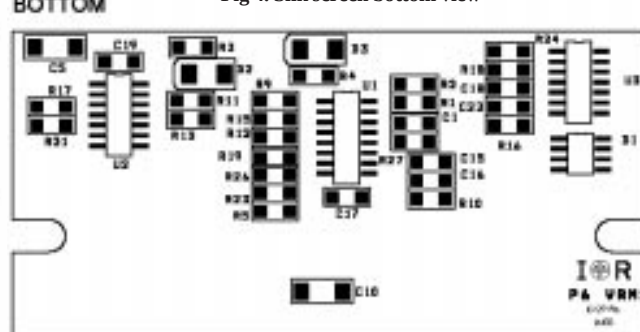
Fig 4. Silk screen bottom view
