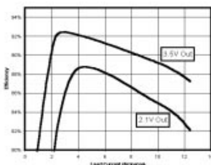
Fig 9. Average Efficiency
