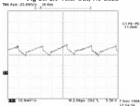
Fig 21. 2.1 Volts Out, No Load
