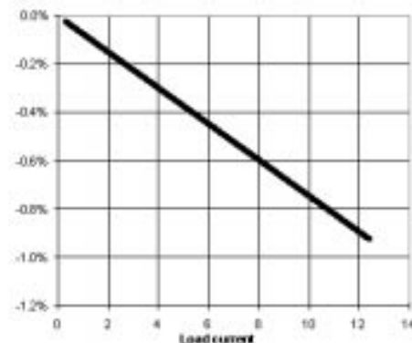
Fig 12. Load Regulation, 3.5 Volts Out
