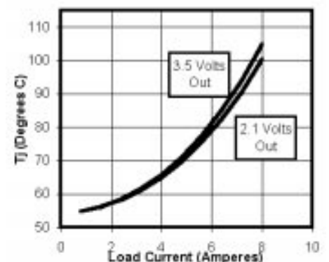
Fig 8. Typical T_j of Q1 @ T_a = 50^\circ\text{C} , still air
