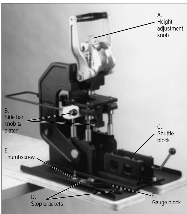
Figure 4. 10960-2000 Hand Press
