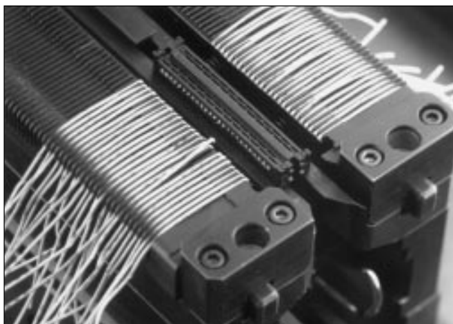
Figure 10. Cut wires
