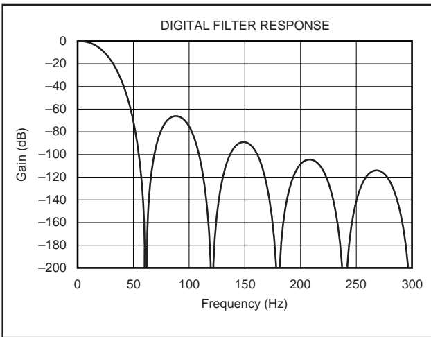
FIGURE 5. Digital Filter Response (60Hz).
