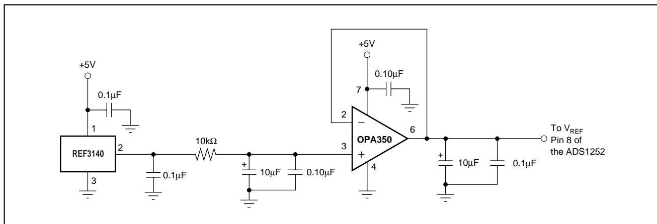
FIGURE 2. Recommended External Voltage Reference Circuit for Best Low-Noise Operation with the ADS1252.
