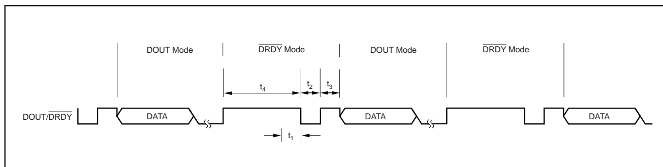
FIGURE 11. DOUT/DRDY Partitioning.
