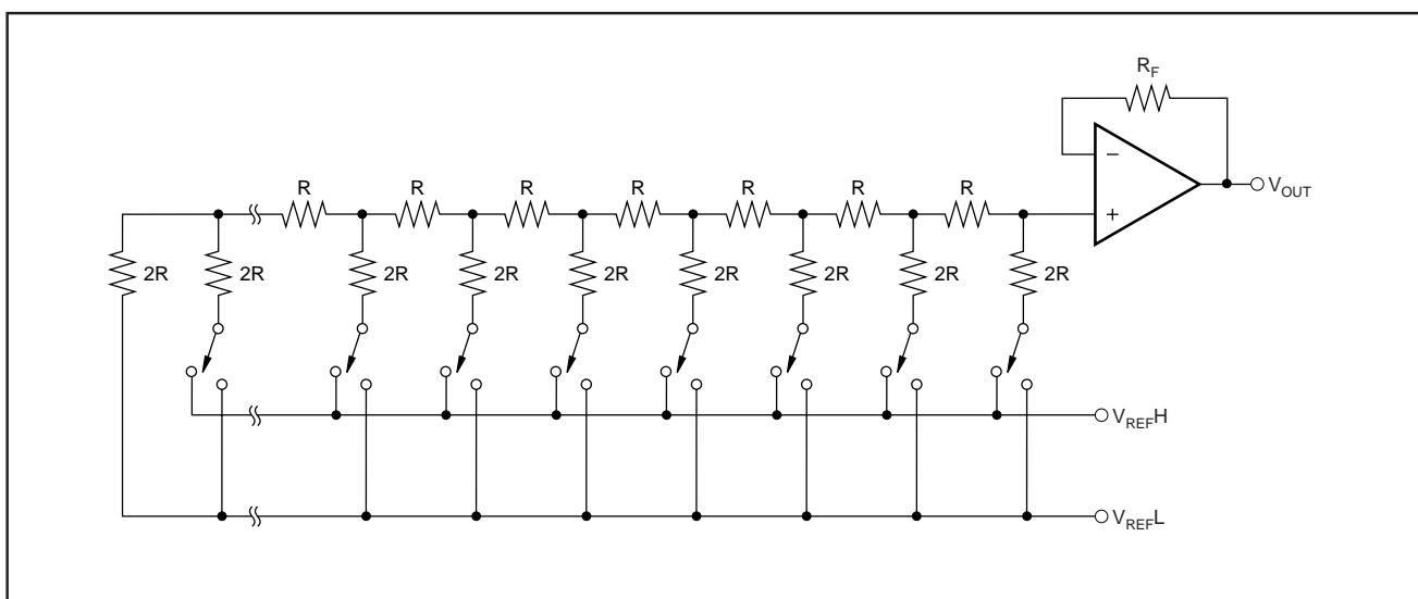
FIGURE 1. DAC7724/25 Architecture.
