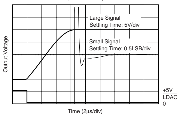
OUTPUT VOLTAGE vs SETTLING TIME (-10V to +10V)
