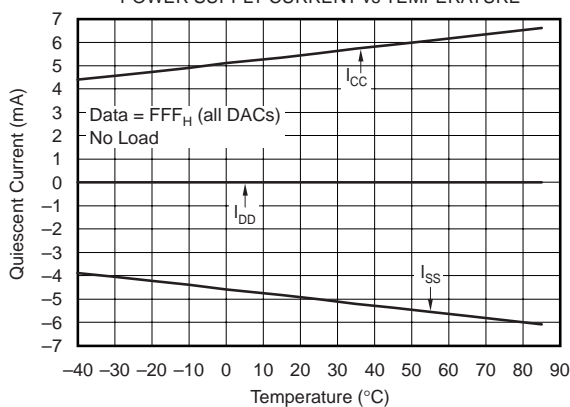
POWER SUPPLY CURRENT vs TEMPERATURE
