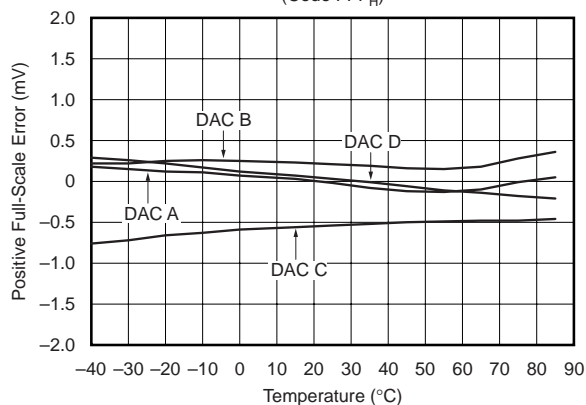
POSITIVE FULL-SCALE ERROR vs TEMPERATURE (Code FFF H )
