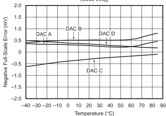
NEGATIVE FULL-SCALE ERROR vs TEMPERATURE (Code 000 H )
