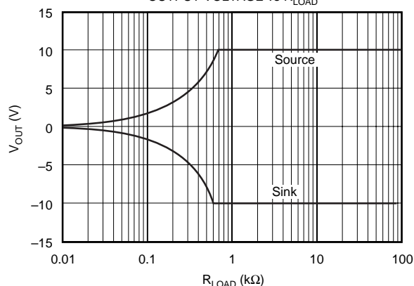
OUTPUT VOLTAGE vs R_{LOAD}
