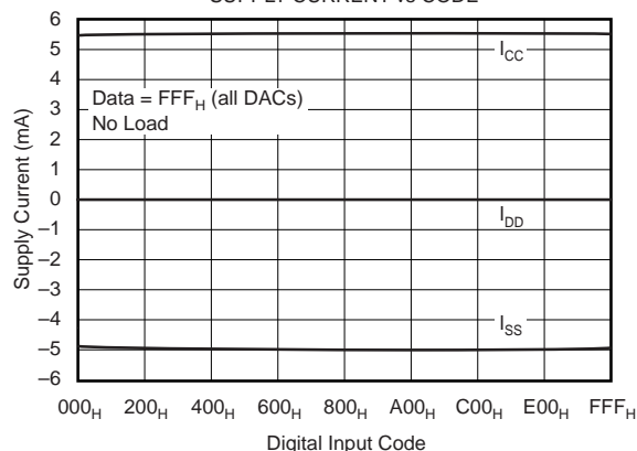
SUPPLY CURRENT vs CODE
