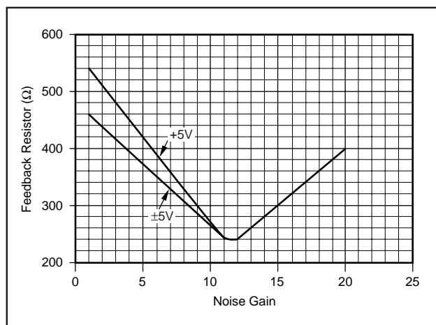
FIGURE 12. Feedback Resistor vs. Noise Gain.
