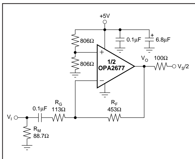
FIGURE 4. AC-Coupled, G = -4 , Single-Supply, Specification and Test Circuit.
