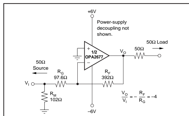
FIGURE 13. Inverting Gain of -4 with Impedance Matching.
