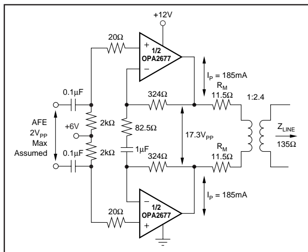
FIGURE 7. HDSL2 Upstream Driver.
