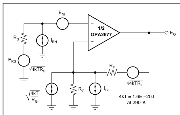
FIGURE 14. Op Amp Noise Analysis Model.
