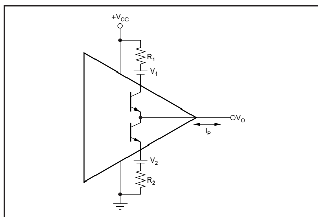
FIGURE 9. Line Driver Headroom Model.
