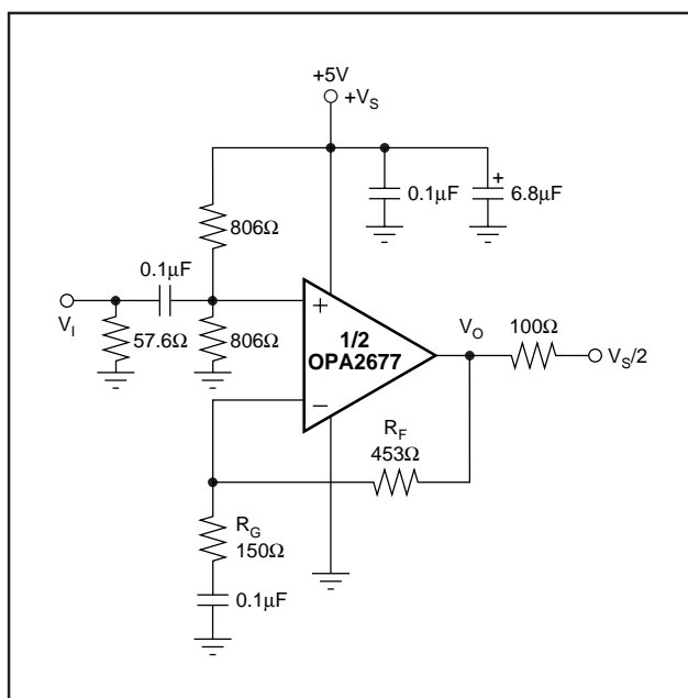
FIGURE 3. AC-Coupled, G = +4 , Single-Supply, Specification and Test Circuit.
