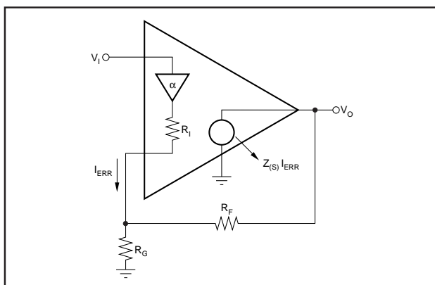
FIGURE 11. Current Feedback Transfer Function Analysis Circuit.
