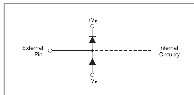
FIGURE 16. Internal ESD Protection.
