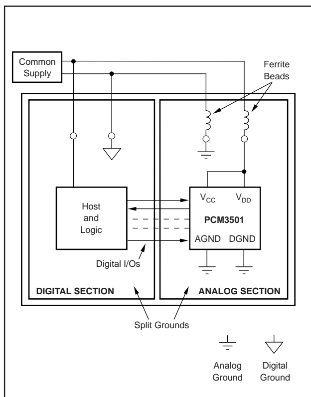
FIGURE 19. PCB Layout Using a Single-Supply or Battery.
