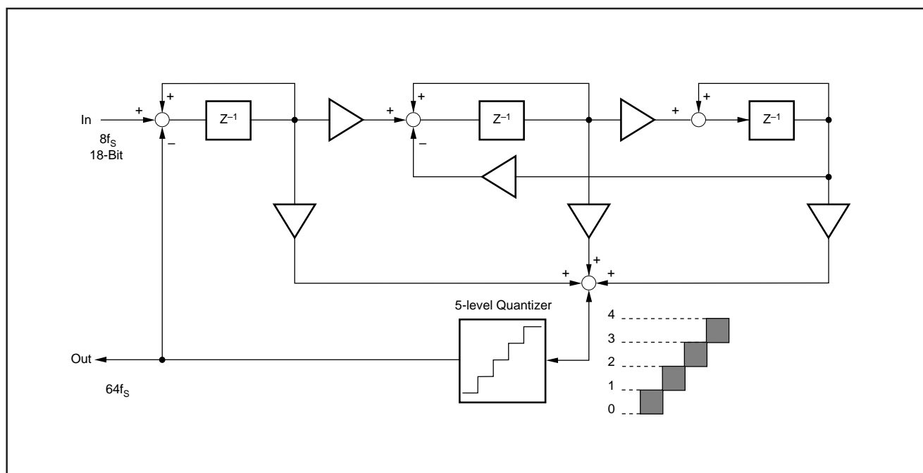
FIGURE 25. 5-Level Delta-Sigma Modulator Block Digram.
