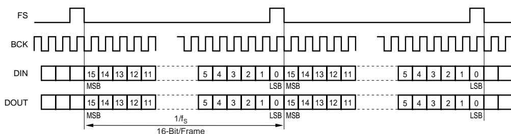
FIGURE 6. Serial Interface Format.
