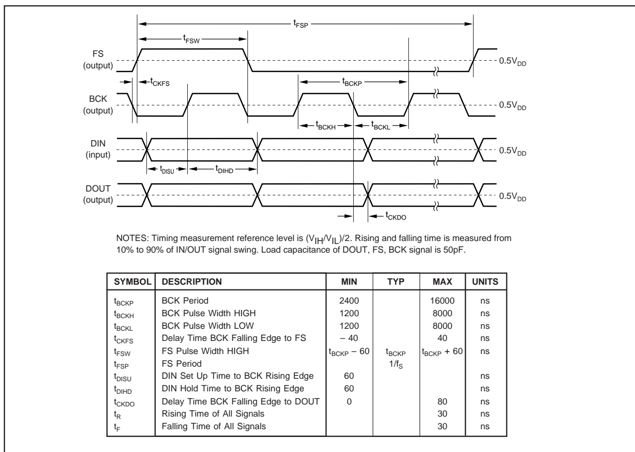
FIGURE 8. Serial Interface Timing for Master Mode.
