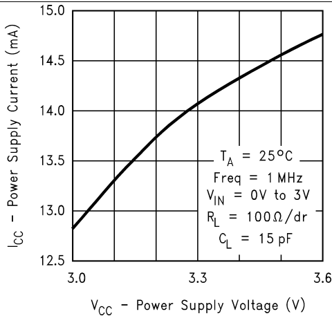
Figure 7. Power Supply Current vs Power Supply Voltage
