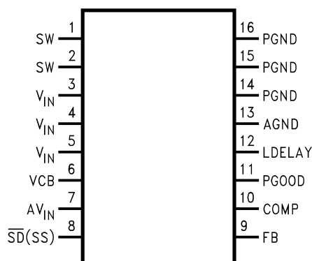
Figure 14. 16-Lead TSSOP (PW) See Package Number PW0016A
