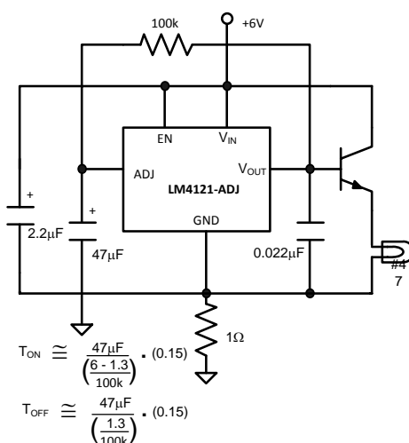
Figure 45. Flasher Circuit
