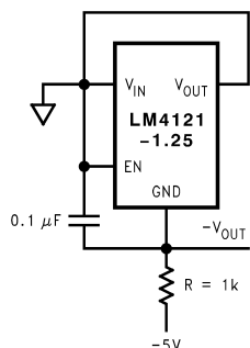
Figure 35. Voltage Reference with Negative Output
