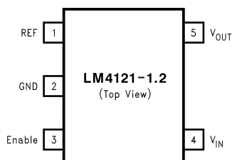
Figure 2. SOT23-5 Surface Mount Package
