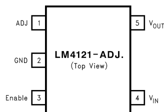
Figure 3. SOT23-5 Surface Mount Package
